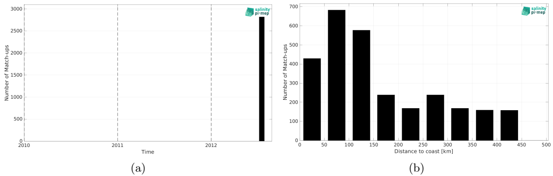
Figure 1: Number of match-ups between TSG (CSIC-UTM) and Aquarius SSS L3 OR v5 - Monthly (NASA-GSFC) SSS as a function of time (a) and as function of the distance to coast (b) over the Gulf Stream Pi-MEP region and for the full satellite product period.
