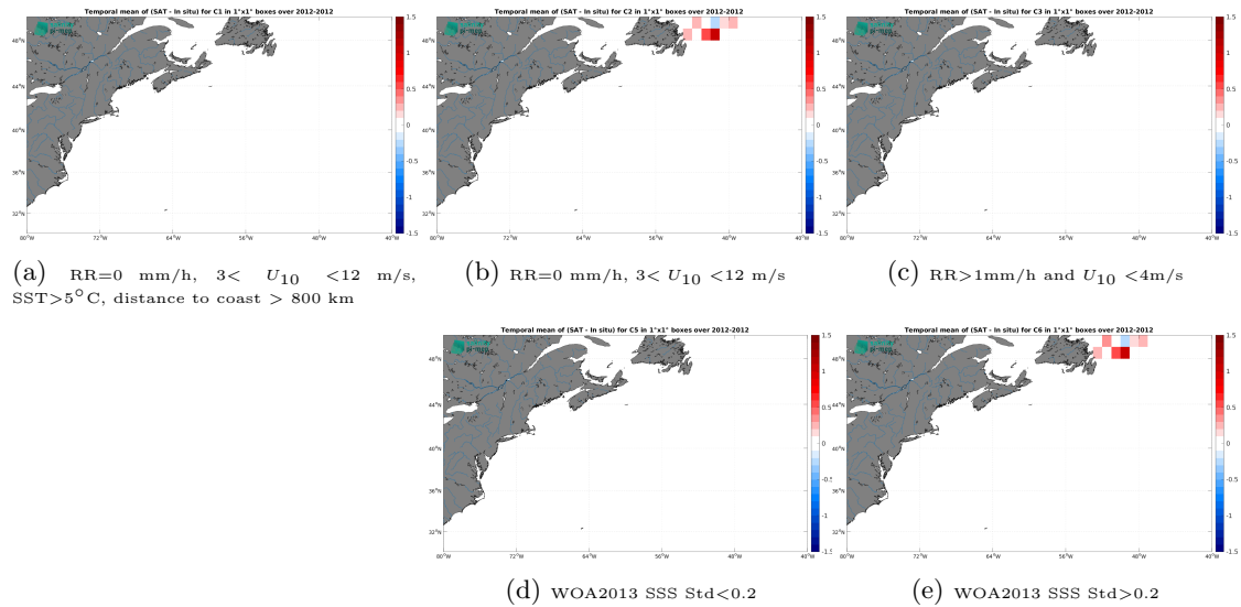
Figure 12: Temporal mean gridded over spatial boxes of size 1^{\circ}\times 1^{\circ} of \Delta\text{SSS} (Aquarius SSS L3 OR v5 - Monthly (NASA-GSFC) - TSG (CSIC-UTM)) for 5 different subdatasets corresponding to:RR=0 mm/h, 3 < U_{10} < 12 m/s, SST >5^{\circ}\text{C} , distance to coast > 800 km (a), RR=0 mm/h, 3 < U_{10} < 12 m/s (b), RR >1 mm/h and U_{10} < 4 m/s (c), WOA2013 SSS Std <0.2 (d), WOA2013 SSS Std >0.2 (e).
