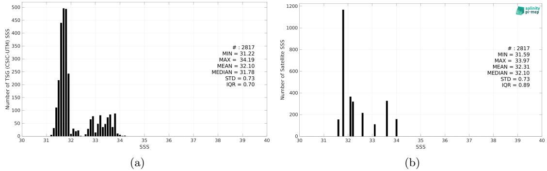
Figure 2: Histograms of SSS from TSG (CSIC-UTM) (a) and Aquarius SSS L3 OR v5 - Monthly (NASA-GSFC) (b) considering all match-up pairs per bins of 0.1 over the Gulf Stream Pi-MEP region and for the full satellite product period.
