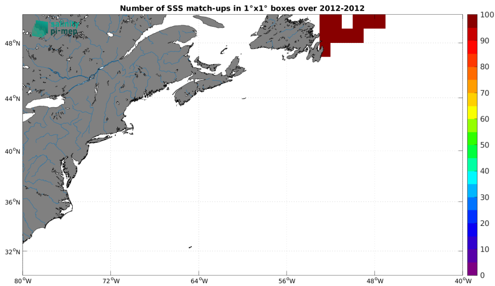
Figure 4: Number of SSS match-ups between TSG (CSIC-UTM) SSS and the Aquarius SSS L3 OR v5 - Monthly (NASA-GSFC) SSS product for the Gulf Stream Pi-MEP region over 1^\circ \times 1^\circ boxes and for the full satellite product period.
