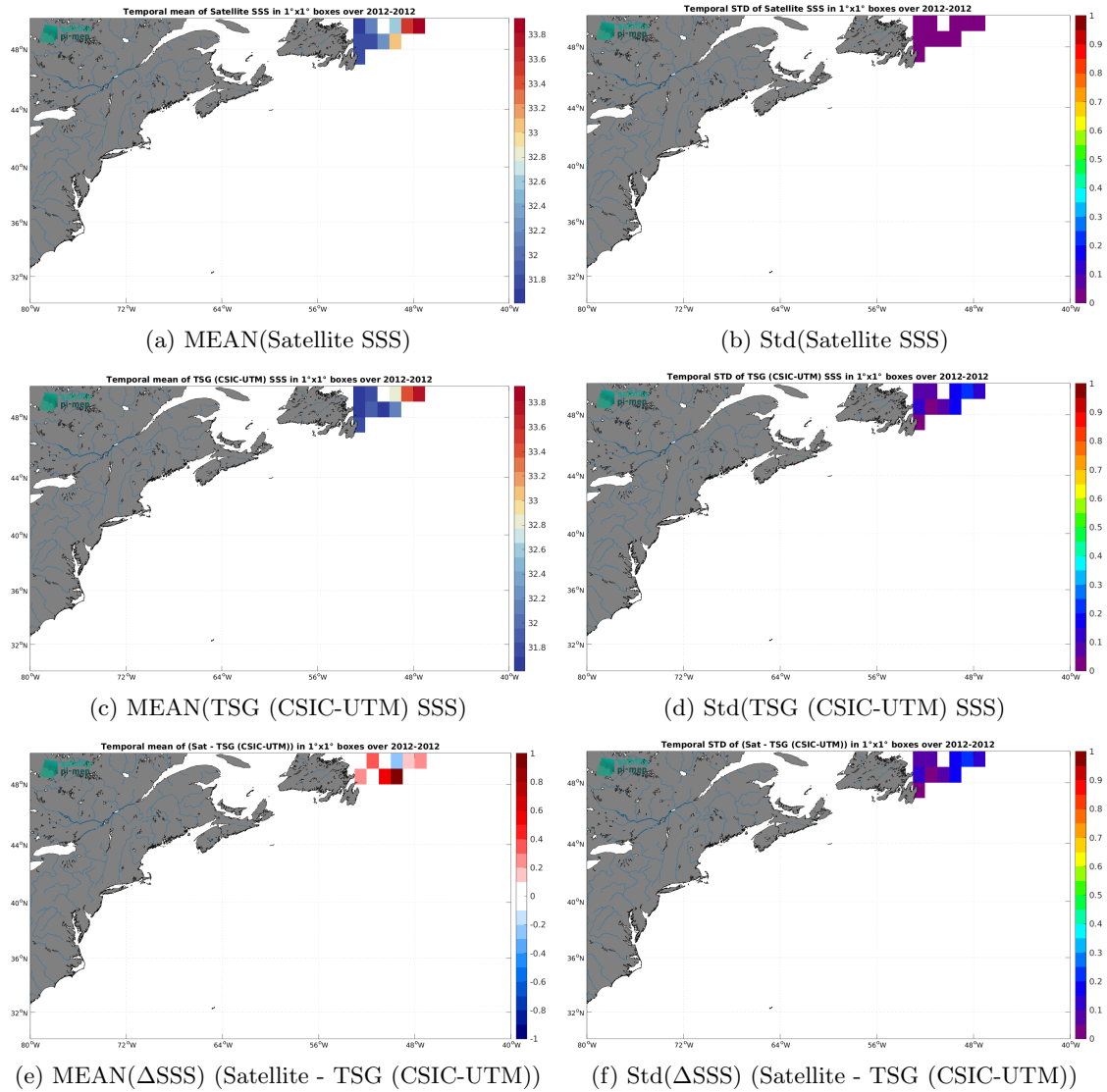
Figure 6: Temporal mean (left) and Std (right) of SSS from Aquarius SSS L3 OR v5 - Monthly (NASA-GSFC) (top), TSG (CSIC-UTM) (middle), and of \Delta SSS (Satellite - TSG (CSIC-UTM)). Only match-up pairs are used to generate these maps.
