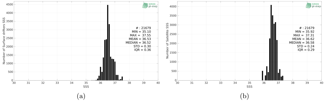
Figure 2: Histograms of SSS from Surface drifters (a) and Aquarius SSS L3 OR v5 - Monthly (NASA-GSFC) (b) considering all match-up pairs per bins of 0.1 over the Gulf Stream Pi-MEP region and for the full satellite product period.
