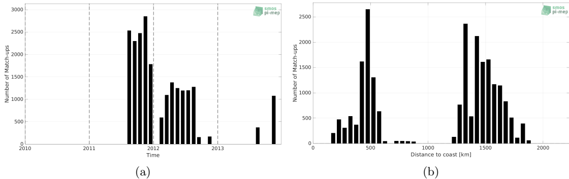
Figure 1: Number of match-ups between Surface drifters and Aquarius SSS L3 OR v5 - Monthly (NASA-GSFC) SSS as a function of time (a) and as function of the distance to coast (b) over the Gulf Stream Pi-MEP region and for the full satellite product period.
