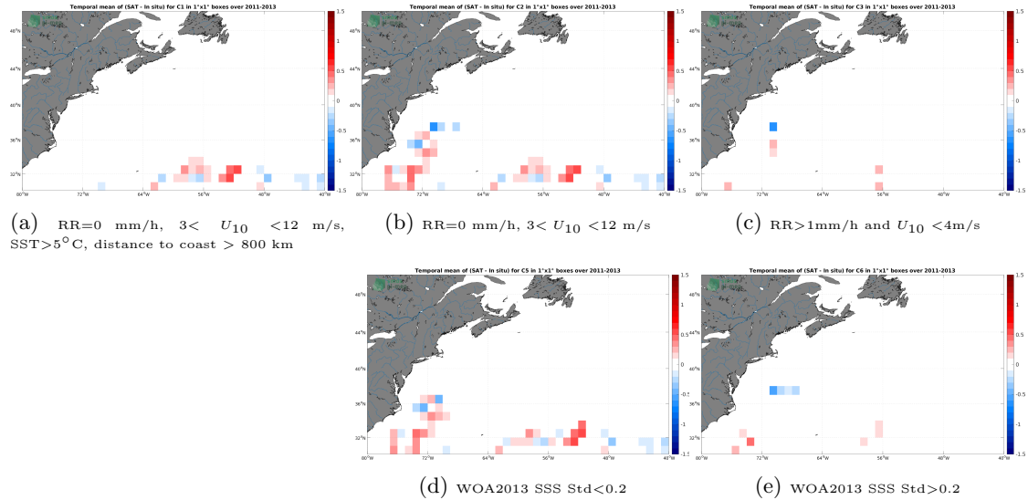
Figure 11: Temporal mean gridded over spatial boxes of size 1^{\circ}\times 1^{\circ} of \Delta\text{SSS} (Aquarius SSS L3 OR v5 - Monthly (NASA-GSFC) - Surface drifters) for 5 different subdatasets corresponding to:RR=0 mm/h, 3 < U_{10} < 12 m/s, SST >5^{\circ}\text{C} , distance to coast > 800 km (a), RR=0 mm/h, 3 < U_{10} < 12 m/s (b), RR >1 mm/h and U_{10} < 4 m/s (c), WOA2013 SSS Std <0.2 (d), WOA2013 SSS Std >0.2 (e).
