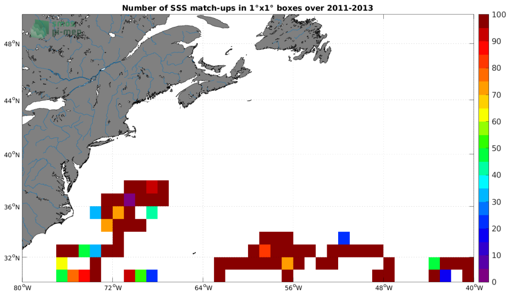
Figure 3: Number of SSS match-ups between Surface drifters SSS and the Aquarius SSS L3 OR v5 - Monthly (NASA-GSFC) SSS product for the Gulf Stream Pi-MEP region over 1^\circ \times 1^\circ boxes and for the full satellite product period.
