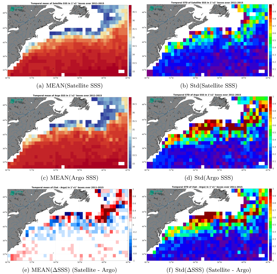
Figure 7: Temporal mean (left) and Std (right) of SSS from Aquarius SSS L3 OR v5 - Monthly (NASA-GSFC) (top), Argo (middle), and of \Delta SSS (Satellite - Argo). Only match-up pairs are used to generate these maps.
