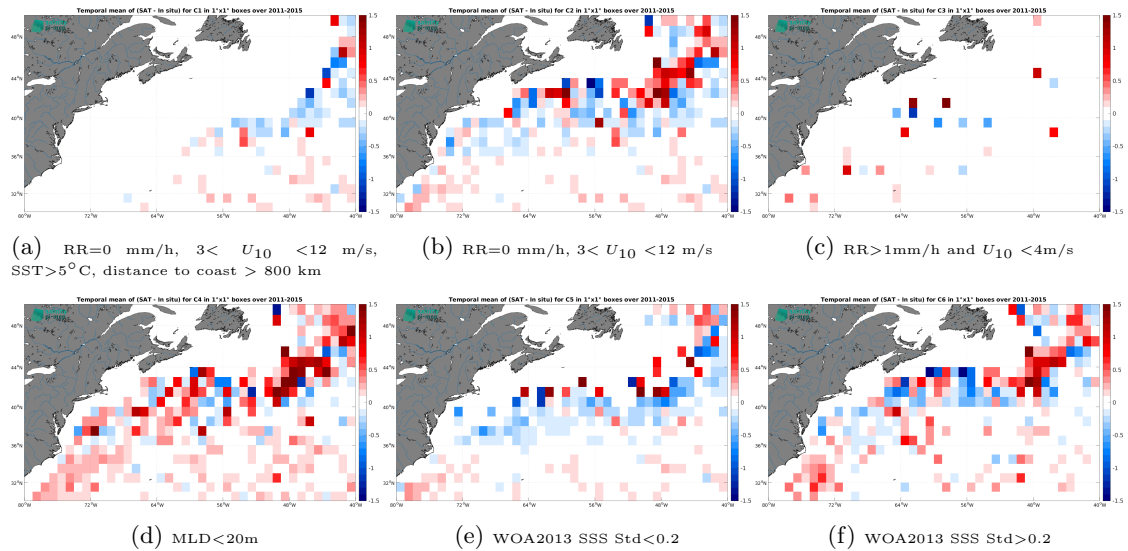
Figure 14: Temporal mean gridded over spatial boxes of size 1^\circ \times 1^\circ of \Delta SSS (Aquarius SSS L3 OR v5 - Monthly (NASA-GSFC) - Argo) for 6 different subdatasets corresponding to:RR=0 mm/h, 3 < U_{10} < 12 m/s, SST >5^\circ C, distance to coast > 800 km (a), RR=0 mm/h, 3 < U_{10} < 12 m/s (b), RR >1 mm/h and U_{10} < 4 m/s (c),MLD <20 m (d),WOA2013 SSS Std <0.2 (e),WOA2013 SSS Std >0.2 (f).
