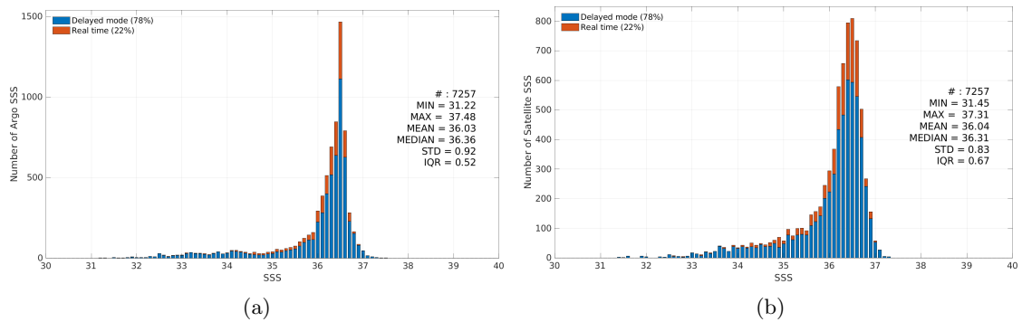
Figure 3: Histograms of SSS from Argo (a) and Aquarius SSS L3 OR v5 - Monthly (NASA-GSFC) (b) considering all match-up pairs per bins of 0.1 over the Gulf Stream Pi-MEP region and for the full satellite product period.
