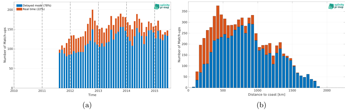
Figure 2: Number of match-ups between Argo and Aquarius SSS L3 OR v5 - Monthly (NASA-GSFC) SSS as a function of time (a) and as function of the distance to coast (b) over the Gulf Stream Pi-MEP region and for the full satellite product period.
