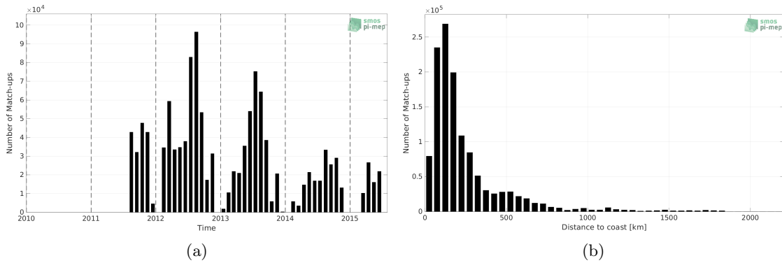
Figure 1: Number of match-ups between TSG (SAMOS) and Aquarius SSS L3 OR v5 - Monthly - Rain mask (NASA-GSFC) SSS as a function of time (a) and as function of the distance to coast (b) over the Gulf Stream Pi-MEP region and for the full satellite product period.
