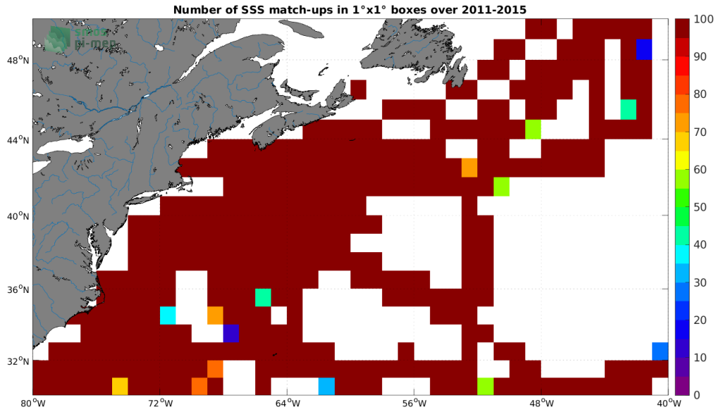
Figure 4: Number of SSS match-ups between TSG (SAMOS) SSS and the Aquarius SSS L3 OR v5 - Monthly - Rain mask (NASA-GSFC) SSS product for the Gulf Stream Pi-MEP region over 1^\circ \times 1^\circ boxes and for the full satellite product period.
