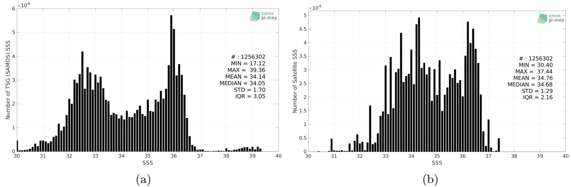
Figure 2: Histograms of SSS from TSG (SAMOS) (a) and Aquarius SSS L3 OR v5 - Monthly - Rain mask (NASA-GSFC) (b) considering all match-up pairs per bins of 0.1 over the Gulf Stream Pi-MEP region and for the full satellite product period.
