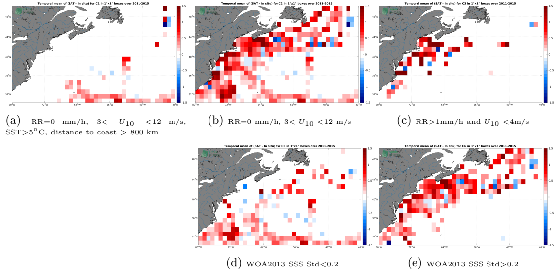
Figure 12: Temporal mean gridded over spatial boxes of size 1^{\circ}\times 1^{\circ} of \Delta\text{SSS} (Aquarius SSS L3 OR v5 - Monthly - Rain mask (NASA-GSFC) - TSG (SAMOS)) for 5 different subdatasets corresponding to:RR=0 mm/h, 3 < U_{10} < 12 m/s, SST >5^{\circ}\text{C} , distance to coast > 800 km (a), RR=0 mm/h, 3 < U_{10} < 12 m/s (b), RR >1 mm/h and U_{10} < 4 m/s (c), WOA2013 SSS Std <0.2 (d), WOA2013 SSS Std >0.2 (e).
