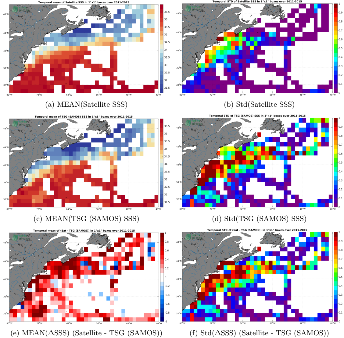
Figure 6: Temporal mean (left) and Std (right) of SSS from Aquarius SSS L3 OR v5 - Monthly - Rain mask (NASA-GSFC) (top), TSG (SAMOS) (middle), and of \Delta SSS (Satellite - TSG (SAMOS)). Only match-up pairs are used to generate these maps.
