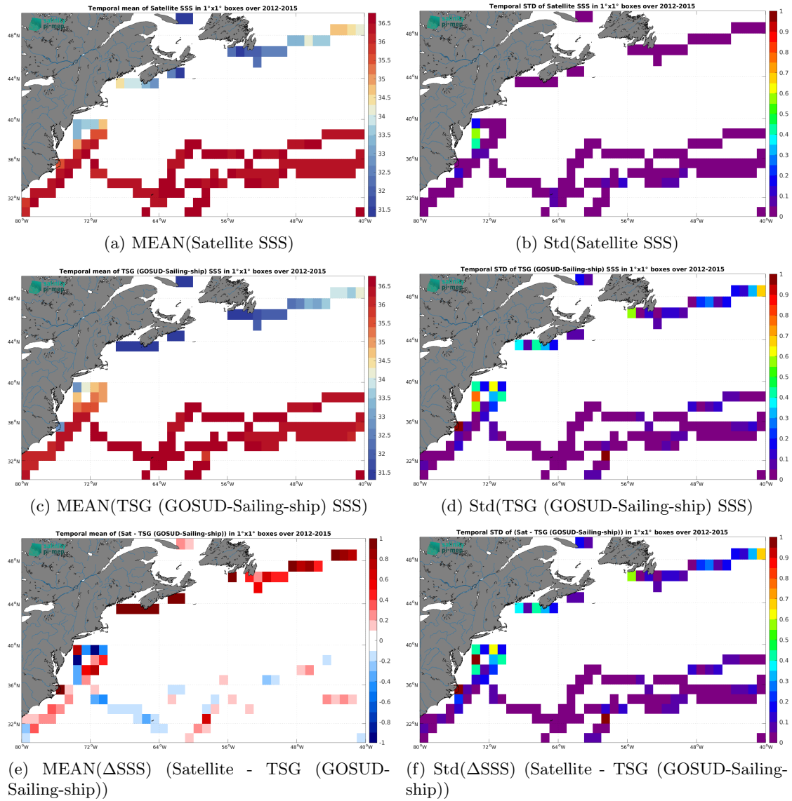
Figure 6: Temporal mean (left) and Std (right) of SSS from Aquarius SSS L3 OR v5 - Monthly - Rain mask (NASA-GSFC) (top), TSG (GOSUD-Sailing-ship) (middle), and of \Delta SSS (Satellite - TSG (GOSUD-Sailing-ship)). Only match-up pairs are used to generate these maps.
