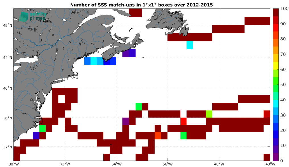
Figure 4: Number of SSS match-ups between TSG (GOSUD-Sailing-ship) SSS and the Aquarius SSS L3 OR v5 - Monthly - Rain mask (NASA-GSFC) SSS product for the Gulf Stream Pi-MEP region over 1^\circ \times 1^\circ boxes and for the full satellite product period.
