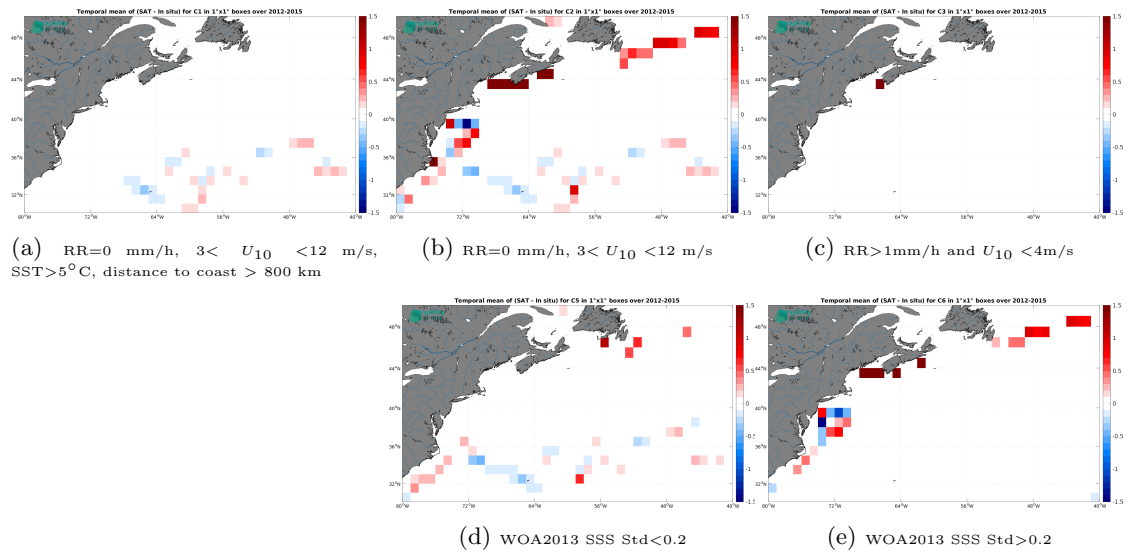
Figure 12: Temporal mean gridded over spatial boxes of size 1^{\circ}\times 1^{\circ} of \Delta SSS (Aquarius SSS L3 OR v5 - Monthly - Rain mask (NASA-GSFC) - TSG (GOSUD-Sailing-ship)) for 5 different subdatasets corresponding to:RR=0 mm/h, 3 < U_{10} < 12 m/s, SST >5^{\circ}\text{C} , distance to coast > 800 km (a), RR=0 mm/h, 3 < U_{10} < 12 m/s (b), RR >1 mm/h and U_{10} < 4 m/s (c), WOA2013 SSS Std <0.2 (d), WOA2013 SSS Std >0.2 (e).
