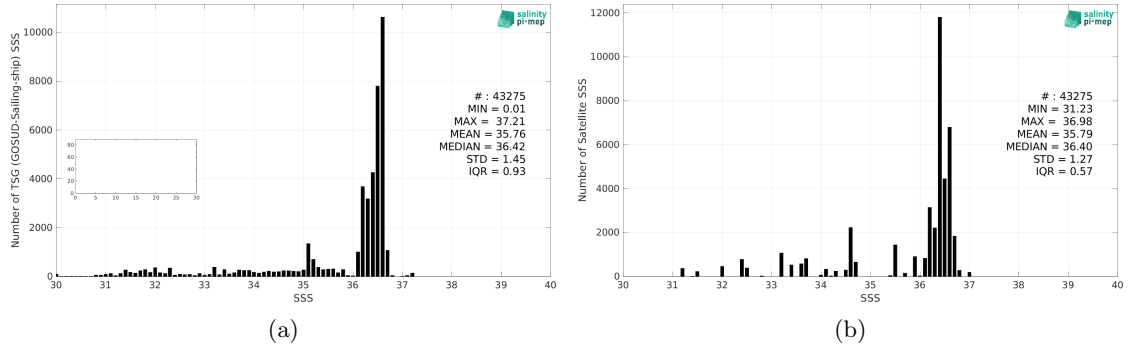
Figure 2: Histograms of SSS from TSG (GOSUD-Sailing-ship) (a) and Aquarius SSS L3 OR v5 - Monthly - Rain mask (NASA-GSFC) (b) considering all match-up pairs per bins of 0.1 over the Gulf Stream Pi-MEP region and for the full satellite product period.
