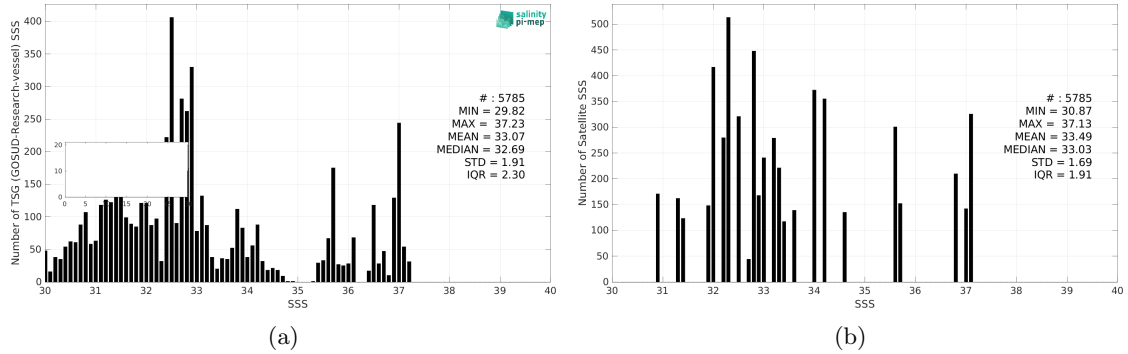
Figure 3: Histograms of SSS from TSG (GOSUD-Research-vessel) (a) and Aquarius SSS L3 OR v5 - Monthly - Rain mask (NASA-GSFC) (b) considering all match-up pairs per bins of 0.1 over the Gulf Stream Pi-MEP region and for the full satellite product period.
