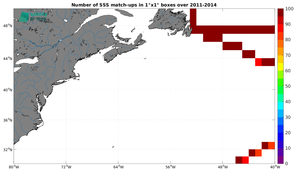
Figure 5: Number of SSS match-ups between TSG (GOSUD-Research-vessel) SSS and the Aquarius SSS L3 OR v5 - Monthly - Rain mask (NASA-GSFC) SSS product for the Gulf Stream Pi-MEP region over 1^\circ \times 1^\circ boxes and for the full satellite product period.
