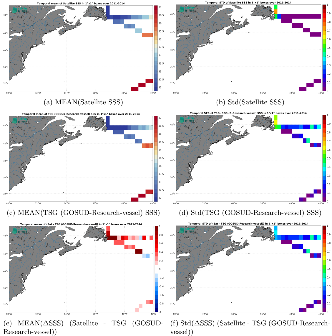
Figure 7: Temporal mean (left) and Std (right) of SSS from Aquarius SSS L3 OR v5 - Monthly - Rain mask (NASA-GSFC) (top), TSG (GOSUD-Research-vessel) (middle), and of \Delta SSS (Satellite - TSG (GOSUD-Research-vessel)). Only match-up pairs are used to generate these maps.
