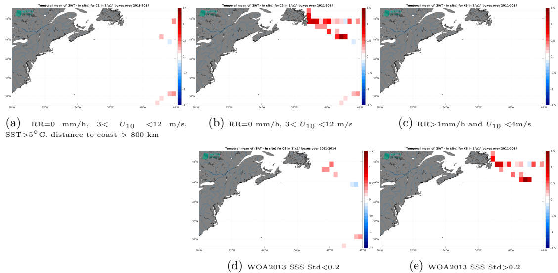
Figure 12: Temporal mean gridded over spatial boxes of size 1^{\circ}\times 1^{\circ} of \Delta SSS (Aquarius SSS L3 OR v5 - Monthly - Rain mask (NASA-GSFC) - TSG (GOSUD-Research-vessel)) for 5 different subdatasets corresponding to:RR=0 mm/h, 3 < U_{10} < 12 m/s, SST > 5^{\circ}\text{C} , distance to coast > 800 km (a), RR=0 mm/h, 3 < U_{10} < 12 m/s (b), RR > 1 mm/h and U_{10} < 4 m/s (c), WOA2013 SSS Std < 0.2 (d), WOA2013 SSS Std > 0.2 (e).
