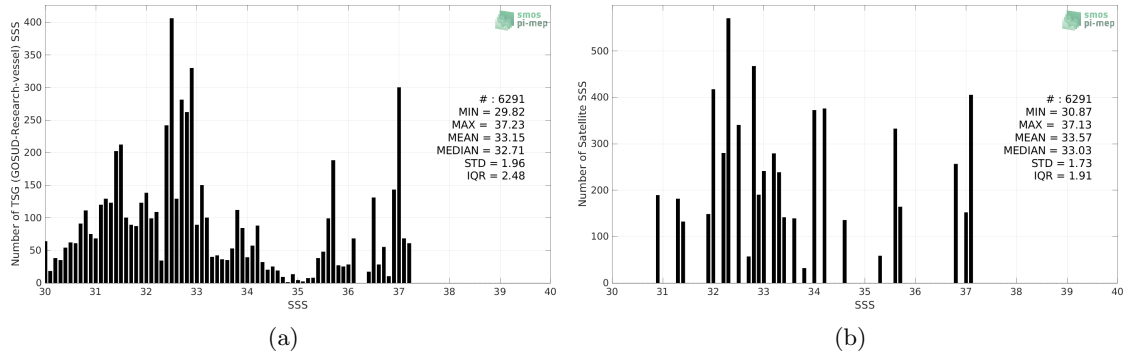
Figure 2: Histograms of SSS from TSG (GOSUD-Research-vessel) (a) and Aquarius SSS L3 OR v5 - Monthly - Rain mask (NASA-GSFC) (b) considering all match-up pairs per bins of 0.1 over the Gulf Stream Pi-MEP region and for the full satellite product period.
