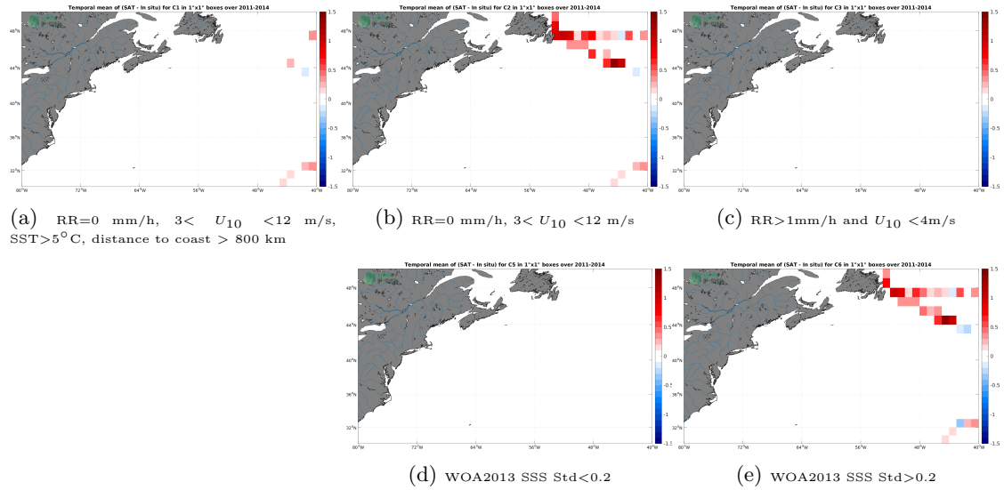
Figure 12: Temporal mean gridded over spatial boxes of size 1^\circ \times 1^\circ of \Delta SSS (Aquarius SSS L3 OR v5 - Monthly - Rain mask (NASA-GSFC) - TSG (GOSUD-Research-vessel)) for 5 different subdatasets corresponding to:RR=0 mm/h, 3 < U_{10} < 12 m/s, SST > 5^\circ\text{C} , distance to coast > 800 km (a), RR=0 mm/h, 3 < U_{10} < 12 m/s (b), RR > 1 mm/h and U_{10} < 4 m/s (c), WOA2013 SSS Std < 0.2 (d), WOA2013 SSS Std > 0.2 (e).
