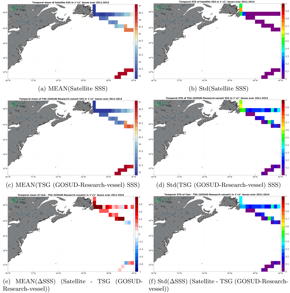
Figure 6: Temporal mean (left) and Std (right) of SSS from Aquarius SSS L3 OR v5 - Monthly - Rain mask (NASA-GSFC) (top), TSG (GOSUD-Research-vessel) (middle), and of \Delta SSS (Satellite - TSG (GOSUD-Research-vessel)). Only match-up pairs are used to generate these maps.
