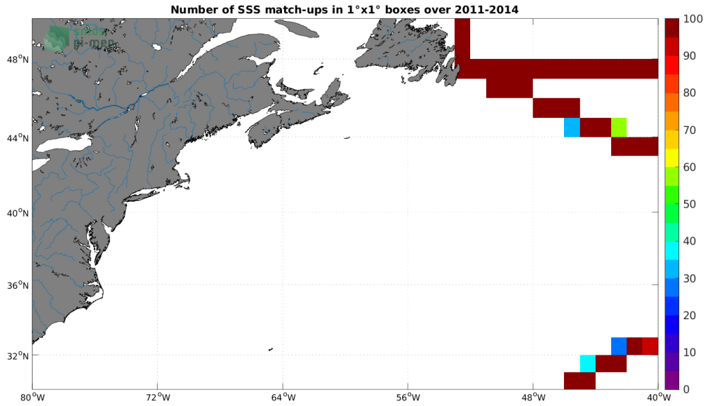
Figure 4: Number of SSS match-ups between TSG (GOSUD-Research-vessel) SSS and the Aquarius SSS L3 OR v5 - Monthly - Rain mask (NASA-GSFC) SSS product for the Gulf Stream Pi-MEP region over 1^\circ \times 1^\circ boxes and for the full satellite product period.
