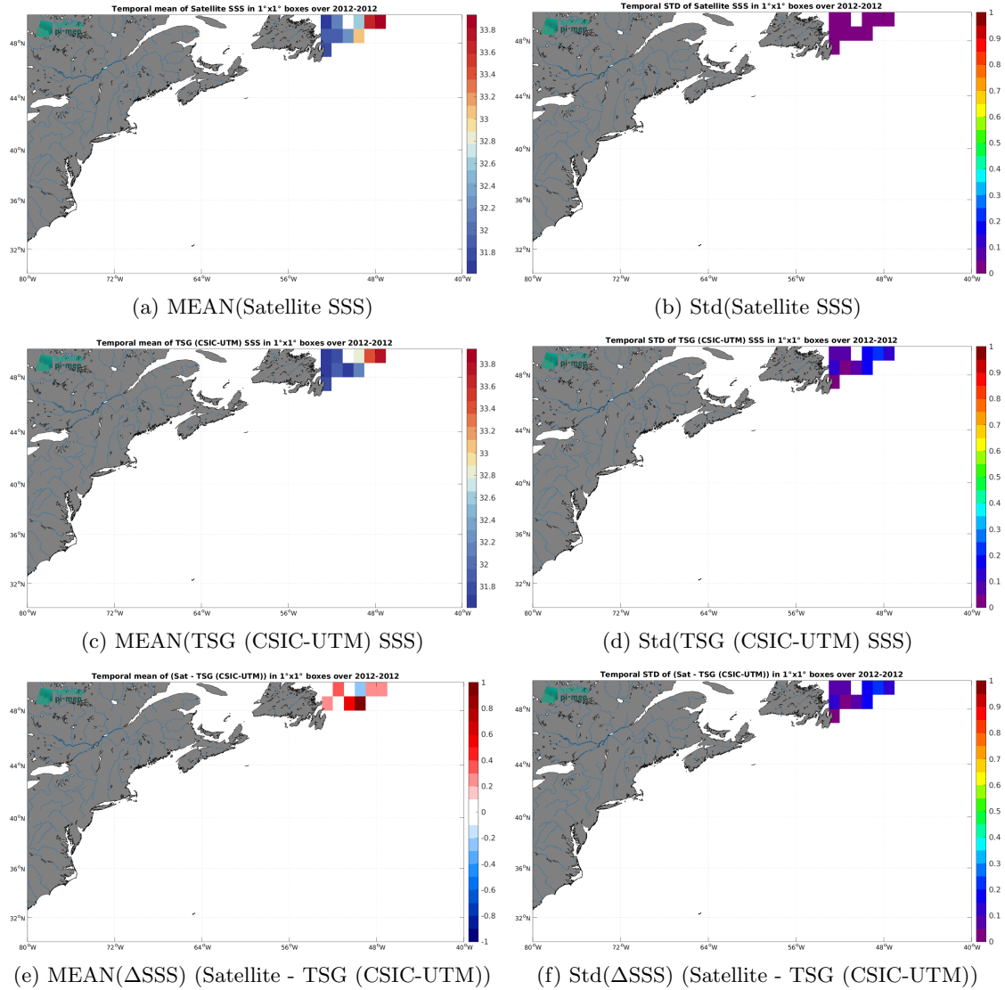
Figure 6: Temporal mean (left) and Std (right) of SSS from Aquarius SSS L3 OR v5 - Monthly - Rain mask (NASA-GSFC) (top), TSG (CSIC-UTM) (middle), and of \Delta SSS (Satellite - TSG (CSIC-UTM)). Only match-up pairs are used to generate these maps.
