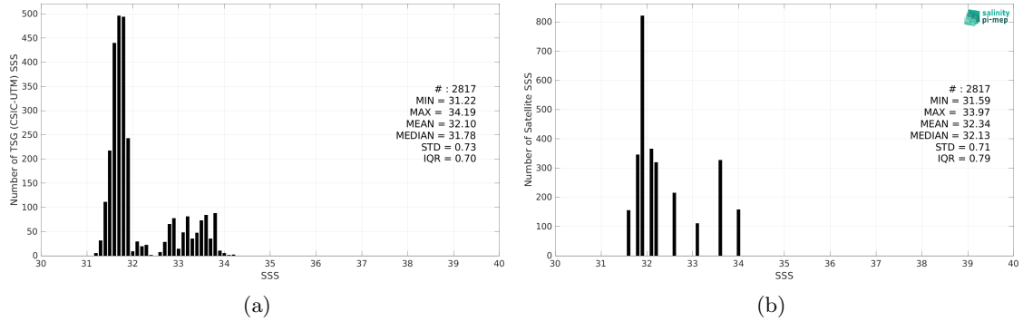
Figure 2: Histograms of SSS from TSG (CSIC-UTM) (a) and Aquarius SSS L3 OR v5 - Monthly - Rain mask (NASA-GSFC) (b) considering all match-up pairs per bins of 0.1 over the Gulf Stream Pi-MEP region and for the full satellite product period.
