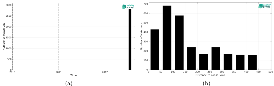
Figure 1: Number of match-ups between TSG (CSIC-UTM) and Aquarius SSS L3 OR v5 - Monthly - Rain mask (NASA-GSFC) SSS as a function of time (a) and as function of the distance to coast (b) over the Gulf Stream Pi-MEP region and for the full satellite product period.
