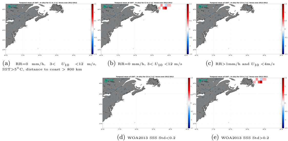
Figure 12: Temporal mean gridded over spatial boxes of size 1^{\circ}\times 1^{\circ} of \Delta\text{SSS} (Aquarius SSS L3 OR v5 - Monthly - Rain mask (NASA-GSFC) - TSG (CSIC-UTM)) for 5 different subdatasets corresponding to:RR=0 mm/h, 3 < U_{10} < 12 m/s, SST >5^{\circ}\text{C} , distance to coast > 800 km (a), RR=0 mm/h, 3 < U_{10} < 12 m/s (b), RR >1 mm/h and U_{10} < 4 m/s (c), WOA2013 SSS Std <0.2 (d), WOA2013 SSS Std >0.2 (e).
