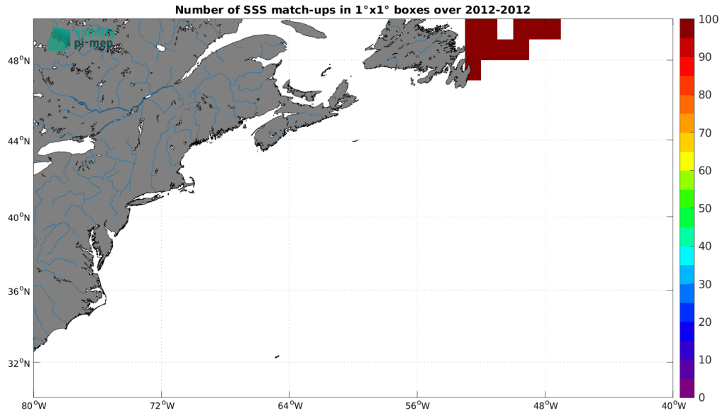
Figure 4: Number of SSS match-ups between TSG (CSIC-UTM) SSS and the Aquarius SSS L3 OR v5 - Monthly - Rain mask (NASA-GSFC) SSS product for the Gulf Stream Pi-MEP region over 1^\circ \times 1^\circ boxes and for the full satellite product period.
