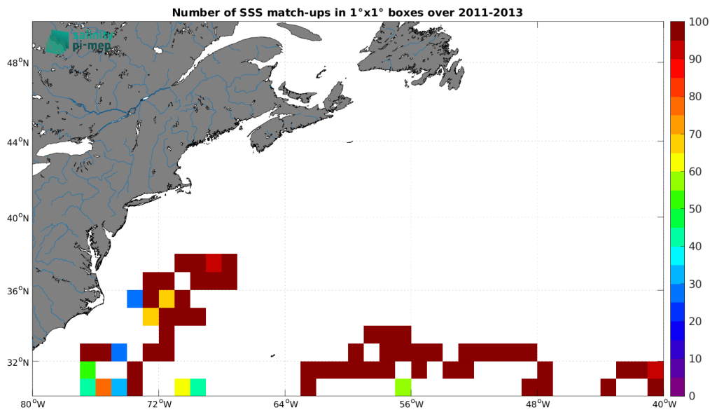
Figure 4: Number of SSS match-ups between Surface drifters SSS and the Aquarius SSS L3 OR v5 - Monthly - Rain mask (NASA-GSFC) SSS product for the Gulf Stream Pi-MEP region over 1^\circ \times 1^\circ boxes and for the full satellite product period.
