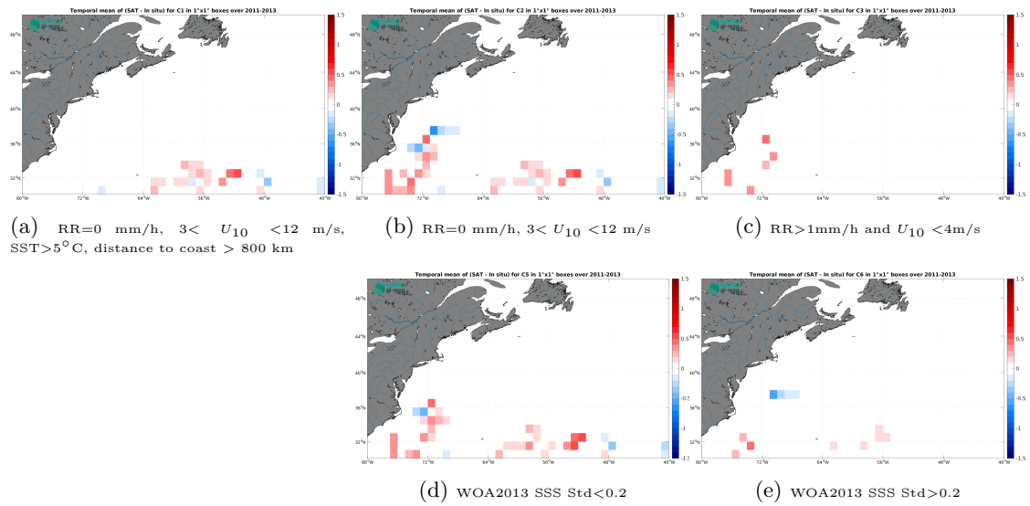
Figure 13: Temporal mean gridded over spatial boxes of size 1^\circ \times 1^\circ of \Delta SSS (Aquarius SSS L3 OR v5 - Monthly - Rain mask (NASA-GSFC) - Surface drifters) for 5 different subdatasets corresponding to:RR=0 mm/h, 3 < U_{10} < 12 m/s, SST >5^\circ\text{C} , distance to coast > 800 km (a), RR=0 mm/h, 3 < U_{10} < 12 m/s (b), RR >1 mm/h and U_{10} < 4 m/s (c), WOA2013 SSS Std <0.2 (d), WOA2013 SSS Std >0.2 (e).
