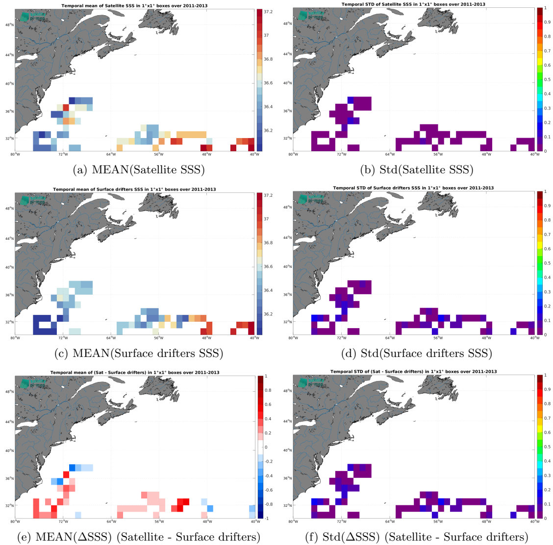
Figure 6: Temporal mean (left) and Std (right) of SSS from Aquarius SSS L3 OR v5 - Monthly - Rain mask (NASA-GSFC) (top), Surface drifters (middle), and of \Delta SSS (Satellite - Surface drifters). Only match-up pairs are used to generate these maps.
