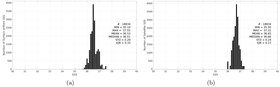
Figure 3: Histograms of SSS from Surface drifters (a) and Aquarius SSS L3 OR v5 - Monthly - Rain mask (NASA-GSFC) (b) considering all match-up pairs per bins of 0.1 over the Gulf Stream Pi-MEP region and for the full satellite product period.
