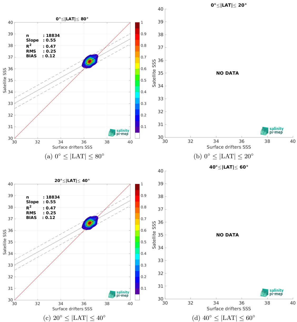
Figure 9: Contour maps of the concentration of Aquarius SSS L3 OR v5 - Monthly - Rain mask (NASA-GSFC) SSS (y-axis) versus Surface drifters SSS (x-axis) at match-up pairs for different latitude bands. For each plot, the red line shows x=y . The black thin and dashed lines indicate a linear fit through the data cloud and the \pm 95\% confidence levels, respectively. The number match-up pairs n , the slope and R^2 coefficient of the linear fit, the root mean square (RMS) and the mean bias between satellite and in situ data are indicated for each latitude band in each plots.
