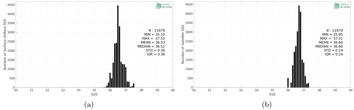
Figure 2: Histograms of SSS from Surface drifters (a) and Aquarius SSS L3 OR v5 - Monthly - Rain mask (NASA-GSFC) (b) considering all match-up pairs per bins of 0.1 over the Gulf Stream Pi-MEP region and for the full satellite product period.
