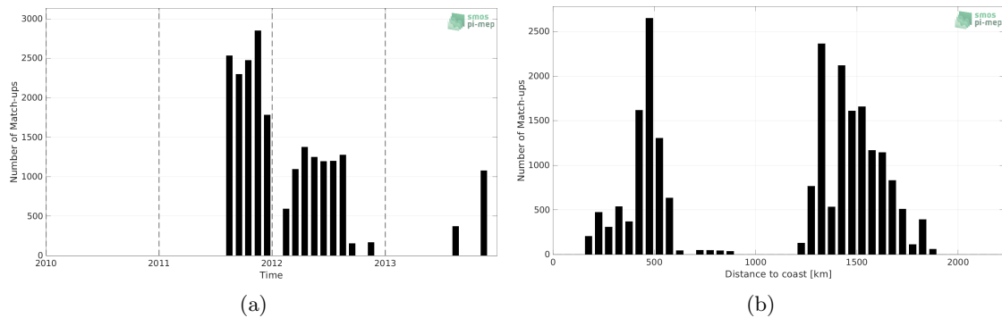
Figure 1: Number of match-ups between Surface drifters and Aquarius SSS L3 OR v5 - Monthly - Rain mask (NASA-GSFC) SSS as a function of time (a) and as function of the distance to coast (b) over the Gulf Stream Pi-MEP region and for the full satellite product period.
