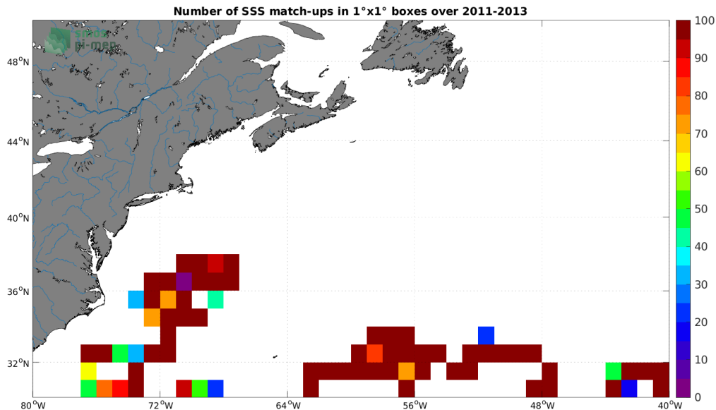
Figure 3: Number of SSS match-ups between Surface drifters SSS and the Aquarius SSS L3 OR v5 - Monthly - Rain mask (NASA-GSFC) SSS product for the Gulf Stream Pi-MEP region over 1^\circ \times 1^\circ boxes and for the full satellite product period.
