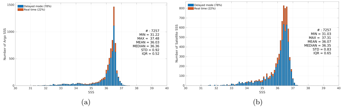
Figure 3: Histograms of SSS from Argo (a) and Aquarius SSS L3 OR v5 - Monthly - Rain mask (NASA-GSFC) (b) considering all match-up pairs per bins of 0.1 over the Gulf Stream Pi-MEP region and for the full satellite product period.
