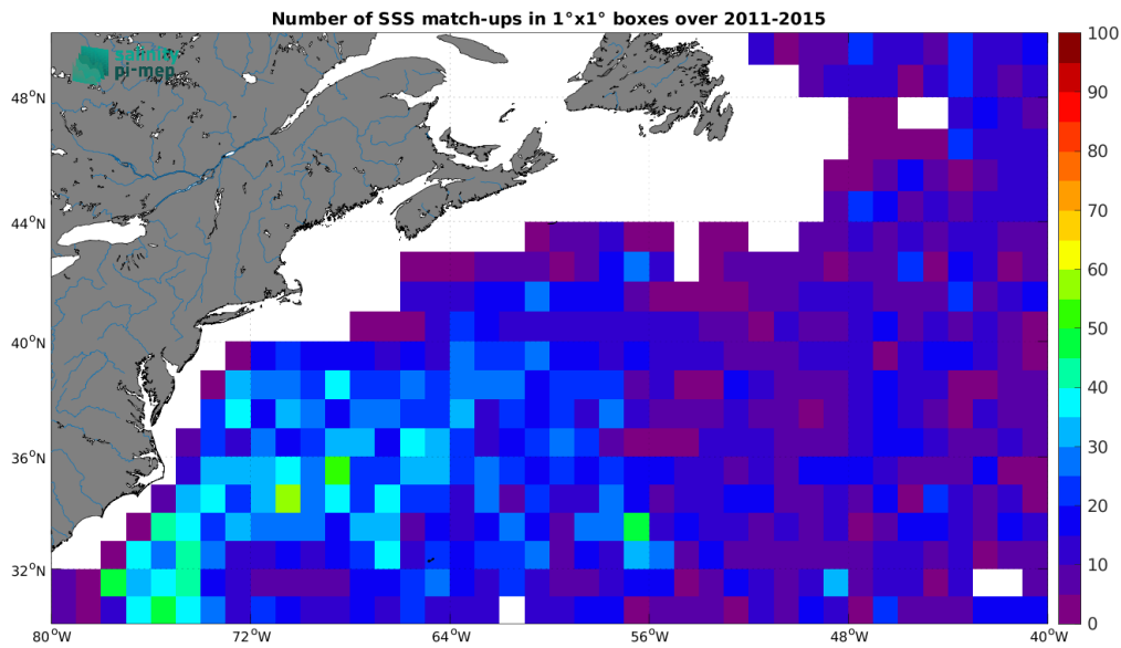
Figure 5: Number of SSS match-ups between Argo SSS and the Aquarius SSS L3 OR v5 - Monthly - Rain mask (NASA-GSFC) SSS product for the Gulf Stream Pi-MEP region over 1^\circ \times 1^\circ boxes and for the full satellite product period.
