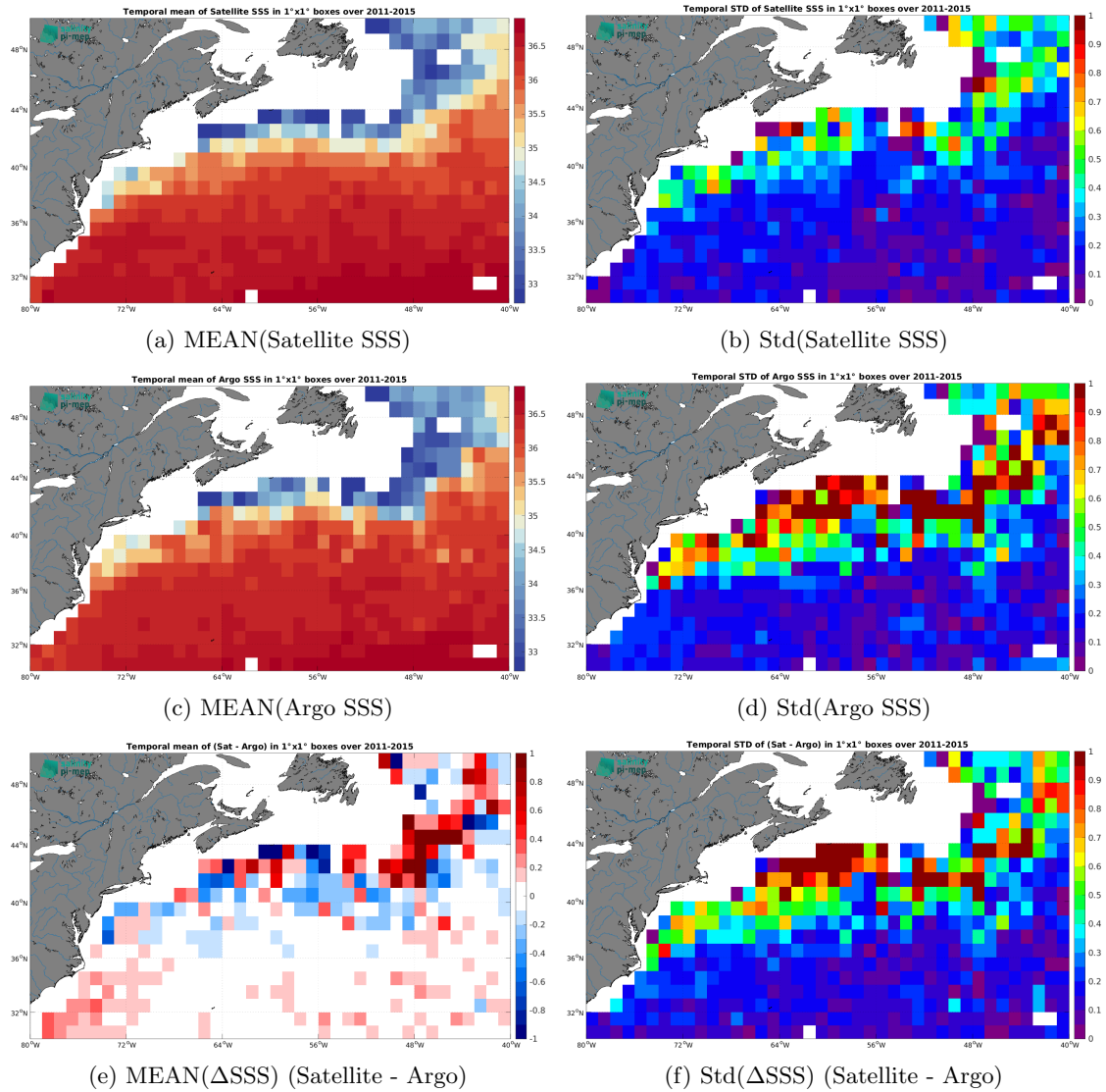
Figure 7: Temporal mean (left) and Std (right) of SSS from Aquarius SSS L3 OR v5 - Monthly - Rain mask (NASA-GSFC) (top), Argo (middle), and of \Delta SSS (Satellite - Argo). Only match-up pairs are used to generate these maps.
