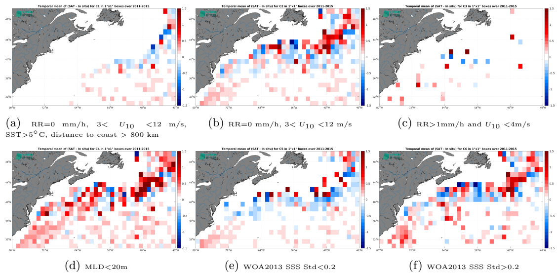
Figure 14: Temporal mean gridded over spatial boxes of size 1^\circ \times 1^\circ of \Delta\text{SSS} (Aquarius SSS L3 OR v5 - Monthly - Rain mask (NASA-GSFC) - Argo) for 6 different subdatasets corresponding to:RR=0 mm/h, 3 < U_{10} < 12 m/s, SST > 5°C, distance to coast > 800 km (a), RR=0 mm/h, 3 < U_{10} < 12 m/s (b), RR > 1mm/h and U_{10} < 4 m/s (c),MLD < 20m (d),WOA2013 SSS Std < 0.2 (e),WOA2013 SSS Std > 0.2 (f).
