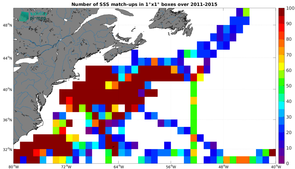
Figure 5: Number of SSS match-ups between TSG (SAMOS) SSS and the Aquarius SSS L3 CAP v5 - 7-Day running (JPL) SSS product for the Gulf Stream Pi-MEP region over 1^\circ \times 1^\circ boxes and for the full satellite product period.
