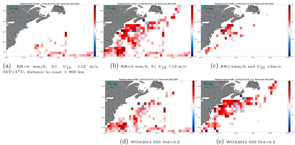
Figure 14: Temporal mean gridded over spatial boxes of size 1^\circ \times 1^\circ of \Delta SSS (Aquarius SSS L3 CAP v5 - 7-Day running (JPL) - TSG (SAMOS)) for 5 different subdatasets corresponding to:RR=0 mm/h, 3 < U_{10} < 12 m/s, SST >5^\circ C, distance to coast > 800 km (a), RR=0 mm/h, 3 < U_{10} < 12 m/s (b), RR >1 mm/h and U_{10} < 4 m/s (c), WOA2013 SSS Std <0.2 (d), WOA2013 SSS Std >0.2 (e).
