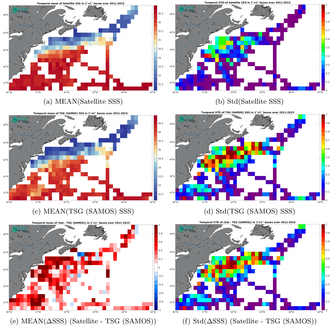
Figure 7: Temporal mean (left) and Std (right) of SSS from Aquarius SSS L3 CAP v5 - 7-Day running (JPL) (top), TSG (SAMOS) (middle), and of \Delta SSS (Satellite - TSG (SAMOS)). Only match-up pairs are used to generate these maps.
