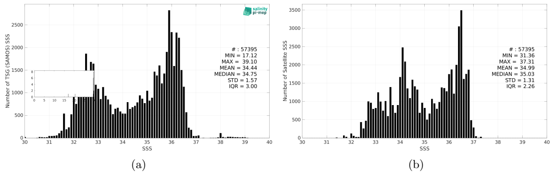
Figure 3: Histograms of SSS from TSG (SAMOS) (a) and Aquarius SSS L3 CAP v5 - 7-Day running (JPL) (b) considering all match-up pairs per bins of 0.1 over the Gulf Stream Pi-MEP region and for the full satellite product period.
