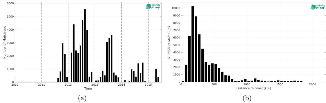
Figure 2: Number of match-ups between TSG (SAMOS) and Aquarius SSS L3 CAP v5 - 7-Day running (JPL) SSS as a function of time (a) and as function of the distance to coast (b) over the Gulf Stream Pi-MEP region and for the full satellite product period.
