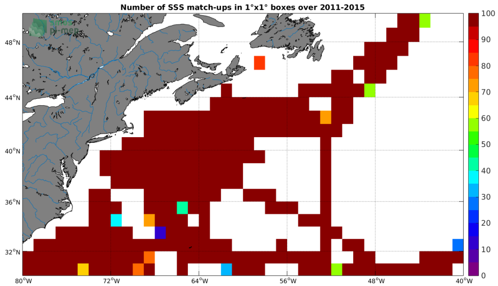
Figure 4: Number of SSS match-ups between TSG-SAMOS SSS and the Aquarius-L3-JPL-V5-7DAY-RUNNING SSS product for the Gulf Stream Pi-MEP region over 1^\circ \times 1^\circ boxes and for the full satellite product period.
