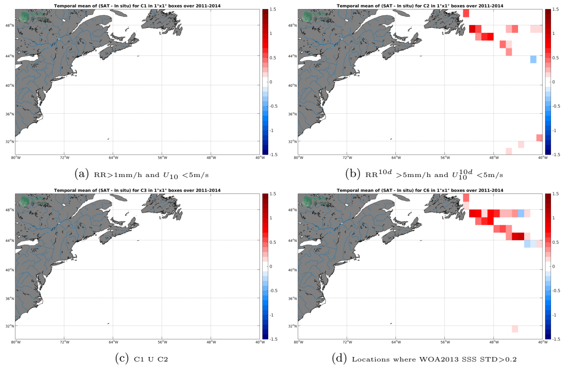
Figure 12: Temporal mean gridded over spatial boxes of size 1^\circ \times 1^\circ of \Delta SSS (Aquarius-L3-JPL-V5-7DAY-RUNNING - TSG-GOSUD-Research-vessel) for 4 different subdatasets corresponding to: RR > 1\text{mm/h} and U_{10} < 5\text{m/s} (a), RR^{10d} > 5\text{mm/h} and U_{10}^{10d} < 5\text{m/s} (b), C1 U C2 (c), Locations where WOA2013 SSS STD > 0.2 (d).
