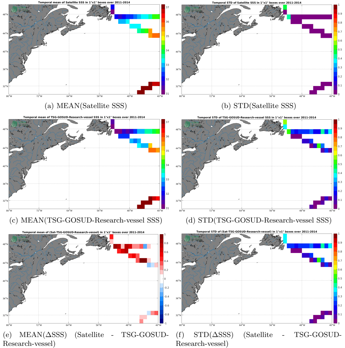
Figure 6: Temporal mean (left) and STD (right) of SSS from Aquarius-L3-JPL-V5-7DAY-RUNNING (top), TSG-GOSUD-Research-vessel (middle), and of \Delta SSS (Satellite - TSG-GOSUD-Research-vessel). Only match-up pairs are used to generate these maps.
