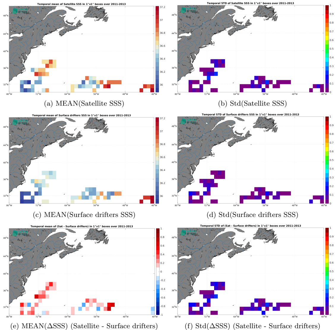
Figure 6: Temporal mean (left) and Std (right) of SSS from Aquarius SSS L3 CAP v5 - 7-Day running (JPL) (top), Surface drifters (middle), and of \Delta SSS (Satellite - Surface drifters). Only match-up pairs are used to generate these maps.
