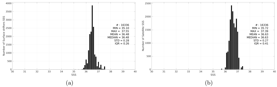
Figure 3: Histograms of SSS from Surface drifters (a) and Aquarius SSS L3 CAP v5 - 7-Day running (JPL) (b) considering all match-up pairs per bins of 0.1 over the Gulf Stream Pi-MEP region and for the full satellite product period.
