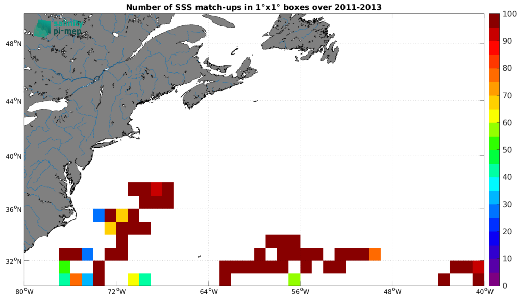
Figure 4: Number of SSS match-ups between Surface drifters SSS and the Aquarius SSS L3 CAP v5 - 7-Day running (JPL) SSS product for the Gulf Stream Pi-MEP region over 1^\circ \times 1^\circ boxes and for the full satellite product period.
