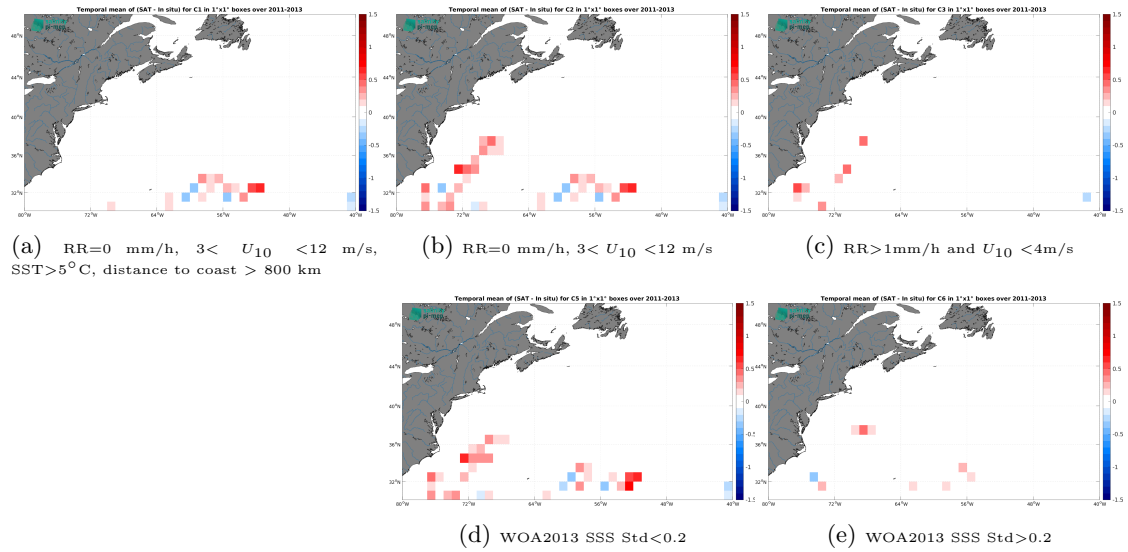
Figure 13: Temporal mean gridded over spatial boxes of size 1^\circ \times 1^\circ of \Delta SSS (Aquarius SSS L3 CAP v5 - 7-Day running (JPL) - Surface drifters) for 5 different subdatasets corresponding to:RR=0 mm/h, 3 < U_{10} < 12 m/s, SST >5^\circ C, distance to coast > 800 km (a), RR=0 mm/h, 3 < U_{10} < 12 m/s (b), RR >1 mm/h and U_{10} < 4 m/s (c), WOA2013 SSS Std <0.2 (d), WOA2013 SSS Std >0.2 (e).
