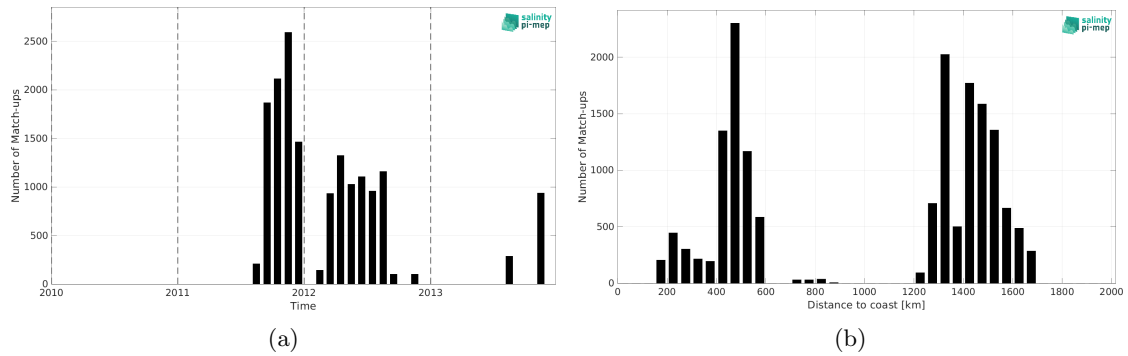
Figure 2: Number of match-ups between Surface drifters and Aquarius SSS L3 CAP v5 - 7-Day running (JPL) SSS as a function of time (a) and as function of the distance to coast (b) over the Gulf Stream Pi-MEP region and for the full satellite product period.
