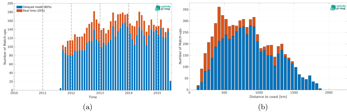
Figure 2: Number of match-ups between Argo and Aquarius SSS L3 CAP v5 - 7-Day running (JPL) SSS as a function of time (a) and as function of the distance to coast (b) over the Gulf Stream Pi-MEP region and for the full satellite product period.
