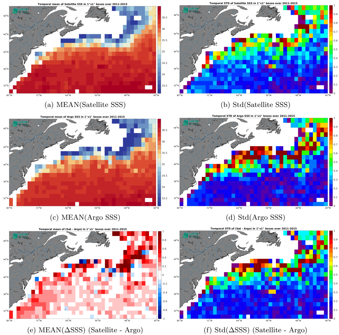
Figure 7: Temporal mean (left) and Std (right) of SSS from Aquarius SSS L3 CAP v5 - 7-Day running (JPL) (top), Argo (middle), and of \Delta SSS (Satellite - Argo). Only match-up pairs are used to generate these maps.
