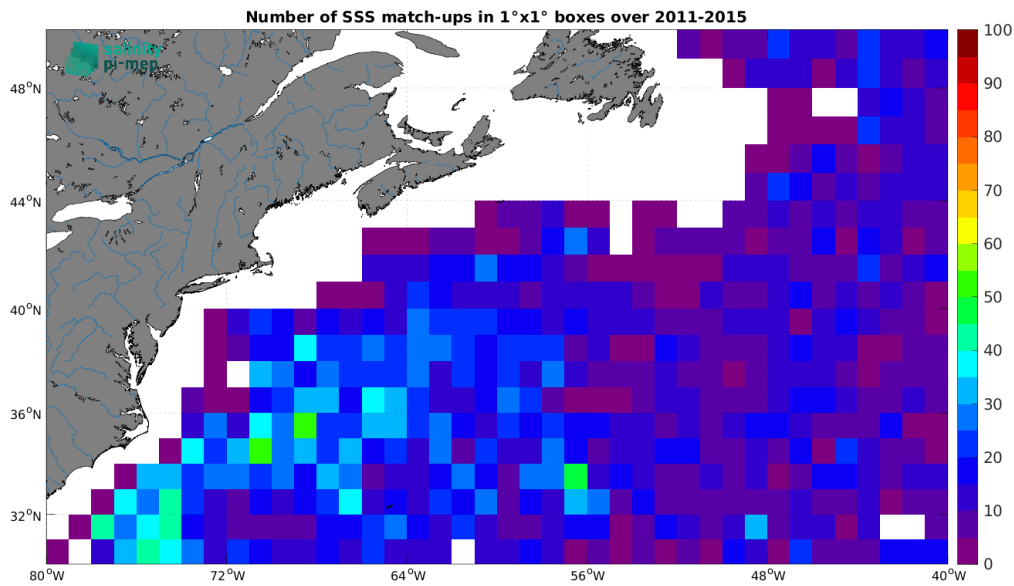
Figure 5: Number of SSS match-ups between Argo SSS and the Aquarius SSS L3 CAP v5 - 7-Day running (JPL) SSS product for the Gulf Stream Pi-MEP region over 1^\circ \times 1^\circ boxes and for the full satellite product period.
