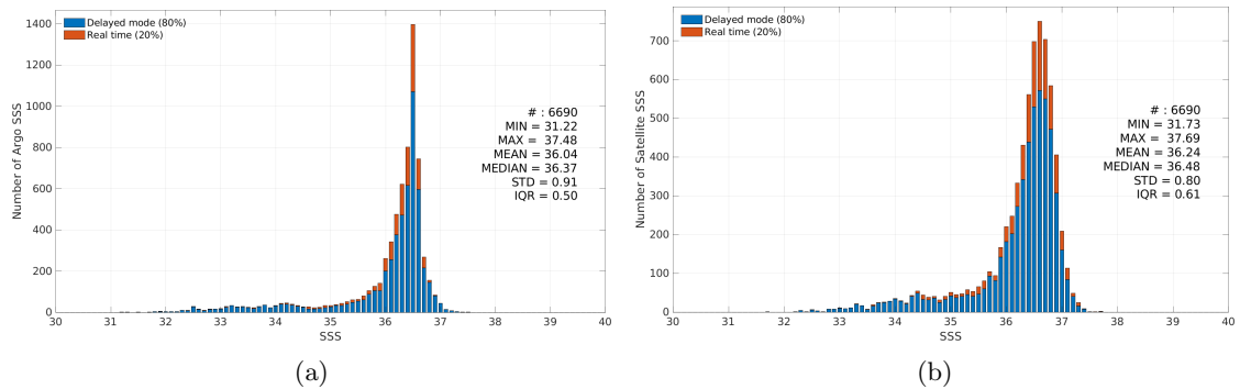
Figure 3: Histograms of SSS from Argo (a) and Aquarius SSS L3 CAP v5 - 7-Day running (JPL) (b) considering all match-up pairs per bins of 0.1 over the Gulf Stream Pi-MEP region and for the full satellite product period.
