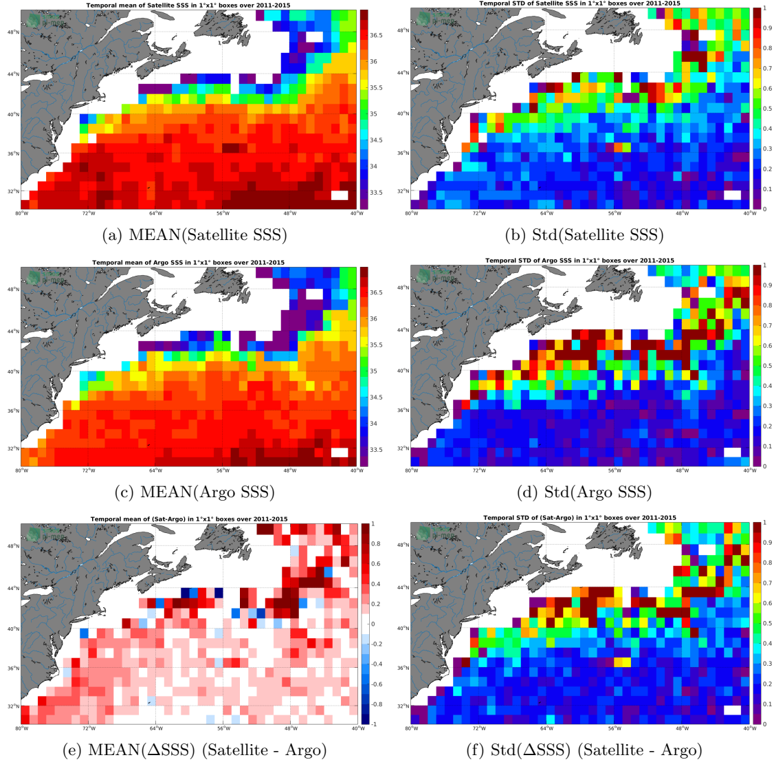
Figure 6: Temporal mean (left) and Std (right) of SSS from Aquarius-L3-JPL-V5-7DAY-RUNNING (top), Argo (middle), and of \Delta\text{SSS} (Satellite - Argo). Only match-up pairs are used to generate these maps.
