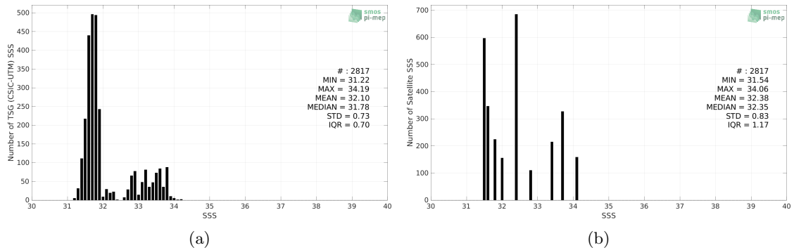
Figure 2: Histograms of SSS from TSG (CSIC-UTM) (a) and Aquarius SSS L3 CAP v5 - Monthly (JPL) (b) considering all match-up pairs per bins of 0.1 over the Gulf Stream Pi-MEP region and for the full satellite product period.
