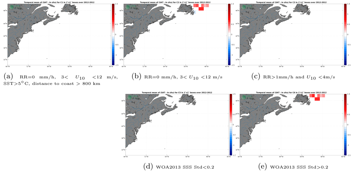
Figure 12: Temporal mean gridded over spatial boxes of size 1^{\circ}\times 1^{\circ} of \Delta\text{SSS} (Aquarius SSS L3 CAP v5 - Monthly (JPL) - TSG (CSIC-UTM)) for 5 different subdatasets corresponding to:RR=0 mm/h, 3 < U_{10} < 12 m/s, SST >5^{\circ}\text{C} , distance to coast > 800 km (a), RR=0 mm/h, 3 < U_{10} < 12 m/s (b), RR >1 mm/h and U_{10} < 4 m/s (c), WOA2013 SSS Std <0.2 (d), WOA2013 SSS Std >0.2 (e).
