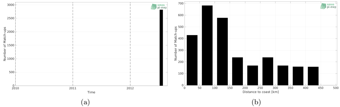
Figure 1: Number of match-ups between TSG (CSIC-UTM) and Aquarius SSS L3 CAP v5 - Monthly (JPL) SSS as a function of time (a) and as function of the distance to coast (b) over the Gulf Stream Pi-MEP region and for the full satellite product period.
