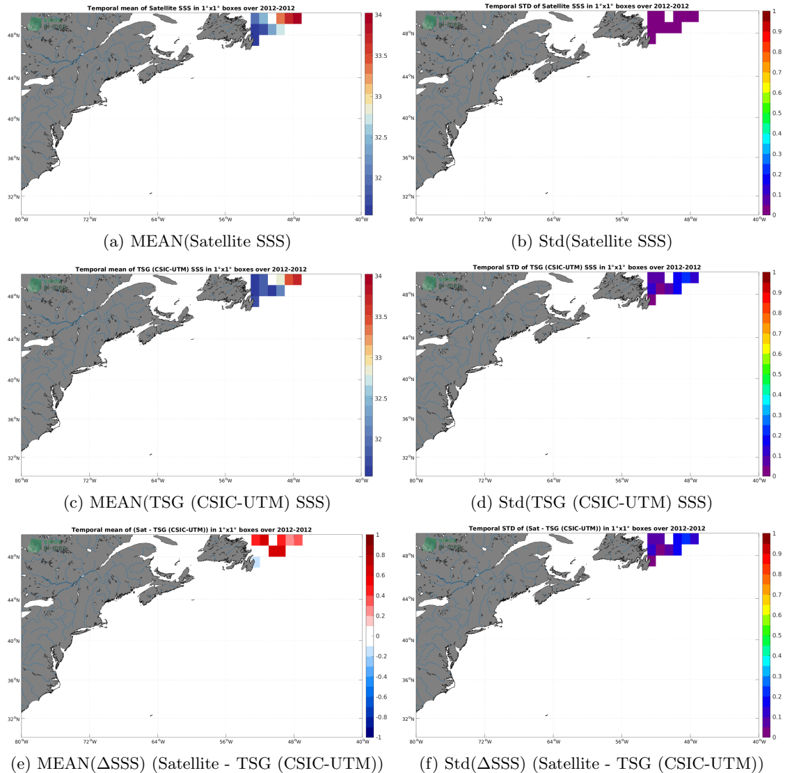
Figure 6: Temporal mean (left) and Std (right) of SSS from Aquarius SSS L3 CAP v5 - Monthly (JPL) (top), TSG (CSIC-UTM) (middle), and of \Delta SSS (Satellite - TSG (CSIC-UTM)). Only match-up pairs are used to generate these maps.
