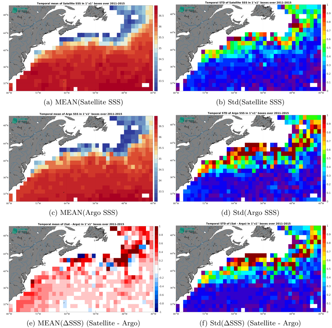
Figure 7: Temporal mean (left) and Std (right) of SSS from Aquarius SSS L3 CAP v5 - Monthly (JPL) (top), Argo (middle), and of \Delta SSS (Satellite - Argo). Only match-up pairs are used to generate these maps.
