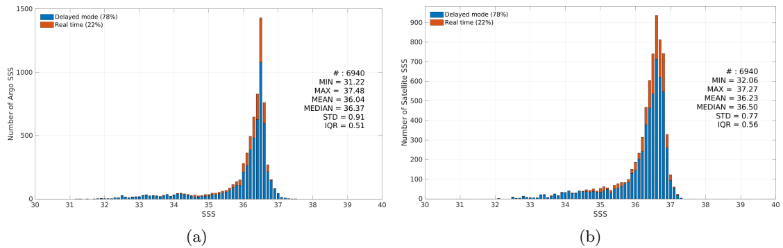
Figure 3: Histograms of SSS from Argo (a) and Aquarius SSS L3 CAP v5 - Monthly (JPL) (b) considering all match-up pairs per bins of 0.1 over the Gulf Stream Pi-MEP region and for the full satellite product period.
