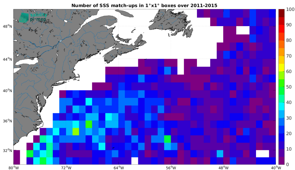
Figure 5: Number of SSS match-ups between Argo SSS and the Aquarius SSS L3 CAP v5 - Monthly (JPL) SSS product for the Gulf Stream Pi-MEP region over 1^\circ \times 1^\circ boxes and for the full satellite product period.
