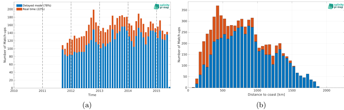
Figure 2: Number of match-ups between Argo and Aquarius SSS L3 CAP v5 - Monthly (JPL) SSS as a function of time (a) and as function of the distance to coast (b) over the Gulf Stream Pi-MEP region and for the full satellite product period.
