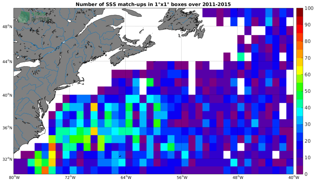
Figure 4: Number of SSS match-ups between Argo SSS and the Aquarius SSS L2-AVERAGED OR v5 (NASA-GSFC) SSS product for the Gulf Stream Pi-MEP region over 1^\circ \times 1^\circ boxes and for the full satellite product period.
