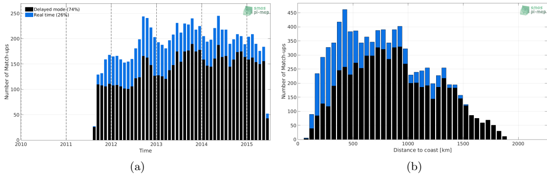
Figure 1: Number of match-ups between Argo and Aquarius SSS L2-AVERAGED OR v5 (NASA-GSFC) SSS as a function of time (a) and as function of the distance to coast (b) over the Gulf Stream Pi-MEP region and for the full satellite product period.
