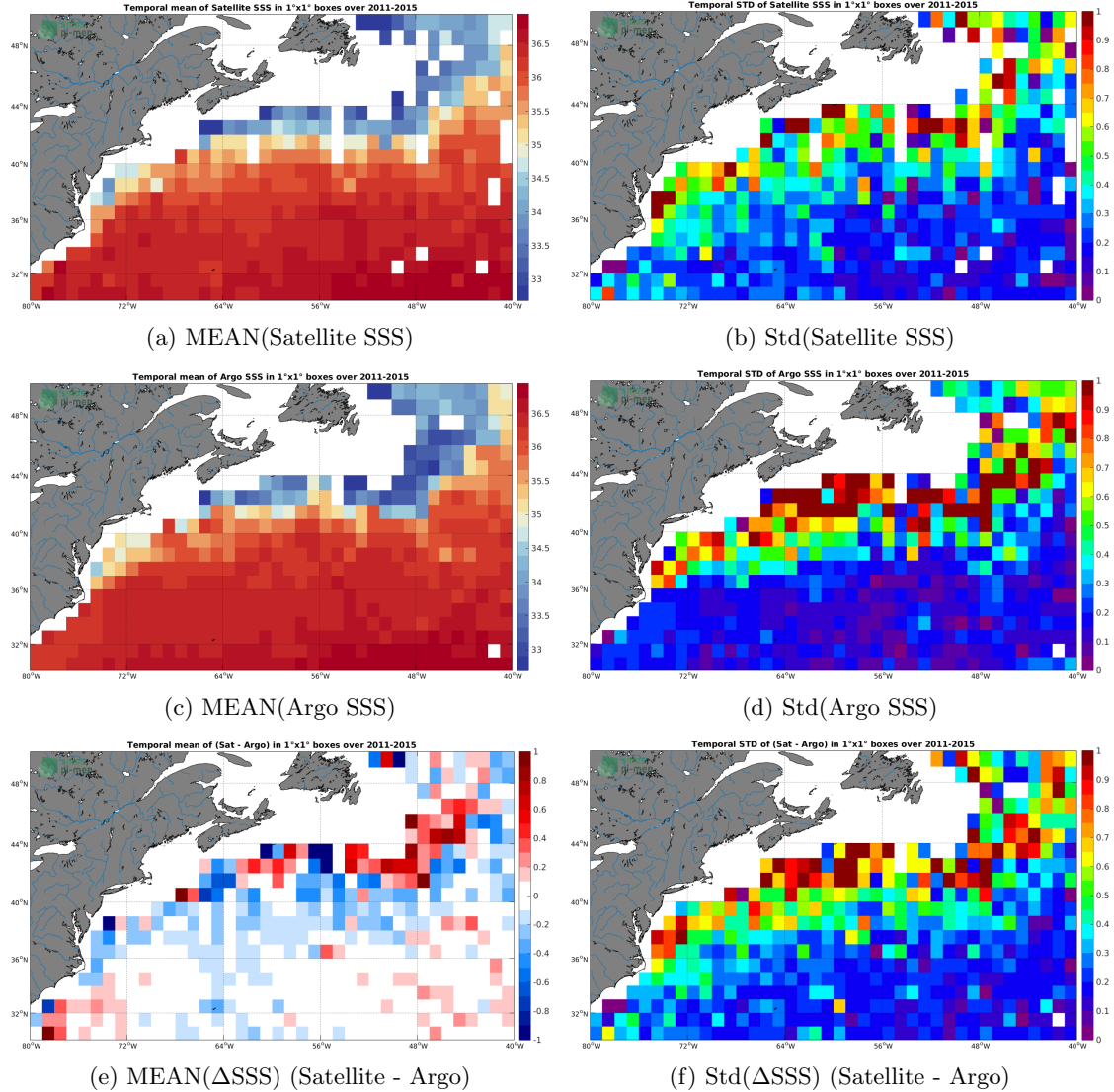
Figure 6: Temporal mean (left) and Std (right) of SSS from Aquarius SSS L2-AVERAGED OR v5 (NASA-GSFC) (top), Argo (middle), and of \Delta SSS (Satellite - Argo). Only match-up pairs are used to generate these maps.
