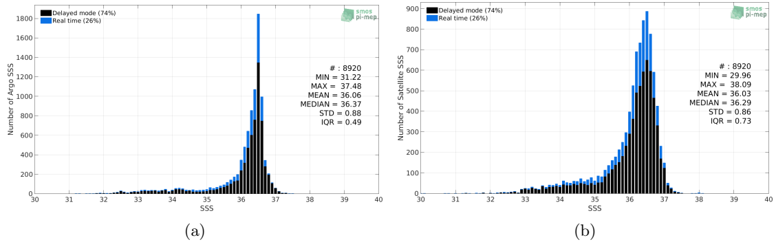
Figure 2: Histograms of SSS from Argo (a) and Aquarius SSS L2-AVERAGED OR v5 (NASA-GSFC) (b) considering all match-up pairs per bins of 0.1 over the Gulf Stream Pi-MEP region and for the full satellite product period.
