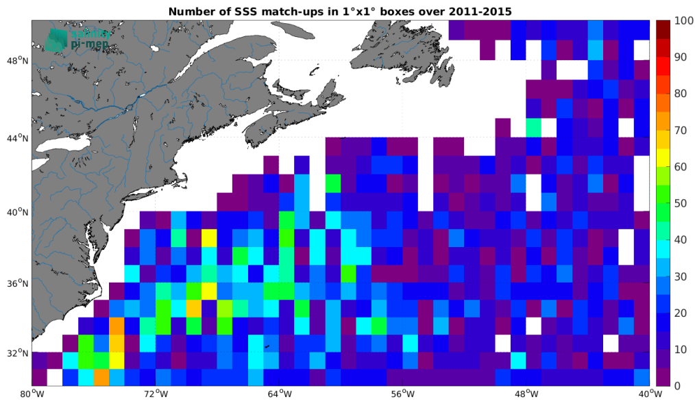
Figure 5: Number of SSS match-ups between Argo SSS and the Aquarius SSS L2-AVERAGED CAP v5 (JPL) SSS product for the Gulf Stream Pi-MEP region over 1^\circ \times 1^\circ boxes and for the full satellite product period.
