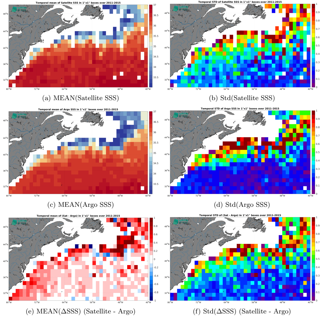
Figure 7: Temporal mean (left) and Std (right) of SSS from Aquarius SSS L2-AVERAGED CAP v5 (JPL) (top), Argo (middle), and of \Delta SSS (Satellite - Argo). Only match-up pairs are used to generate these maps.
