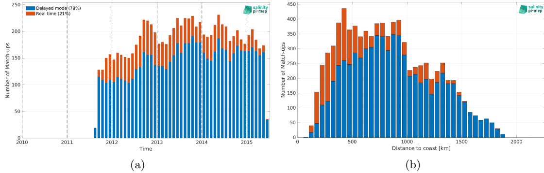
Figure 2: Number of match-ups between Argo and Aquarius SSS L2-AVERAGED CAP v5 (JPL) SSS as a function of time (a) and as function of the distance to coast (b) over the Gulf Stream Pi-MEP region and for the full satellite product period.
