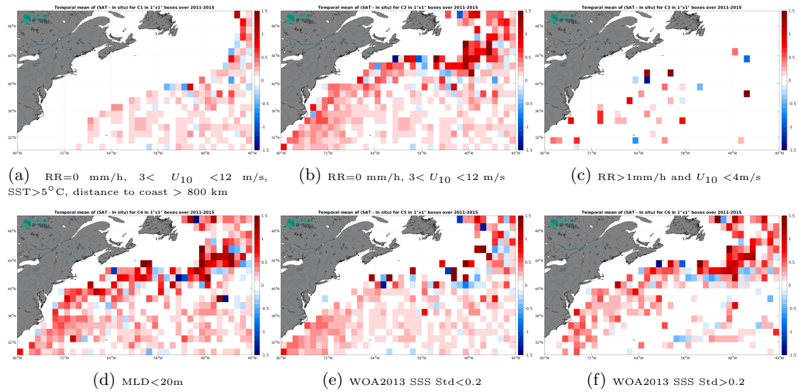
Figure 14: Temporal mean gridded over spatial boxes of size 1^\circ \times 1^\circ of \Delta SSS (Aquarius SSS L2-AVERAGED CAP v5 (JPL) - Argo) for 6 different subdatasets corresponding to:RR=0 mm/h, 3 < U_{10} < 12 m/s, SST >5^\circ C, distance to coast > 800 km (a), RR=0 mm/h, 3 < U_{10} < 12 m/s (b), RR >1 mm/h and U_{10} < 4 m/s (c),MLD <20 m (d),WOA2013 SSS Std <0.2 (e),WOA2013 SSS Std >0.2 (f).
