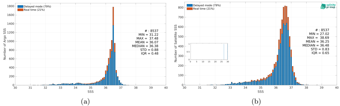
Figure 3: Histograms of SSS from Argo (a) and Aquarius SSS L2-AVERAGED CAP v5 (JPL) (b) considering all match-up pairs per bins of 0.1 over the Gulf Stream Pi-MEP region and for the full satellite product period.
