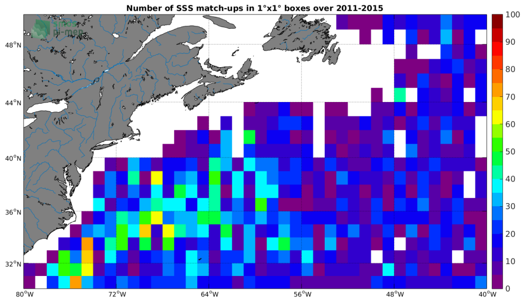
Figure 4: Number of SSS match-ups between Argo SSS and the Aquarius SSS L2-AVERAGED CAP v5 (JPL) SSS product for the Gulf Stream Pi-MEP region over 1^\circ \times 1^\circ boxes and for the full satellite product period.
