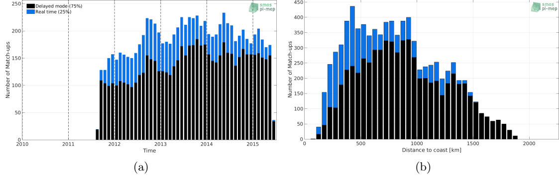
Figure 1: Number of match-ups between Argo and Aquarius SSS L2-AVERAGED CAP v5 (JPL) SSS as a function of time (a) and as function of the distance to coast (b) over the Gulf Stream Pi-MEP region and for the full satellite product period.
