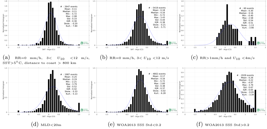
Figure 13: Normalized histogram of \Delta\text{SSS} (Aquarius SSS L2-AVERAGED CAP v5 (JPL) - Argo) for 6 different subdatasets corresponding to: RR=0 mm/h, 3 < U_{10} < 12 m/s, SST>5°C, distance to coast > 800 km (a), RR=0 mm/h, 3 < U_{10} < 12 m/s (b), RR>1mm/h and U_{10} < 4 m/s (c), MLD<20m (d), WOA2013 SSS Std<0.2 (e), WOA2013 SSS Std>0.2 (f).
