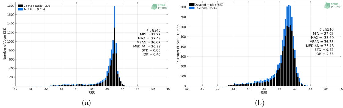
Figure 2: Histograms of SSS from Argo (a) and Aquarius SSS L2-AVERAGED CAP v5 (JPL) (b) considering all match-up pairs per bins of 0.1 over the Gulf Stream Pi-MEP region and for the full satellite product period.
