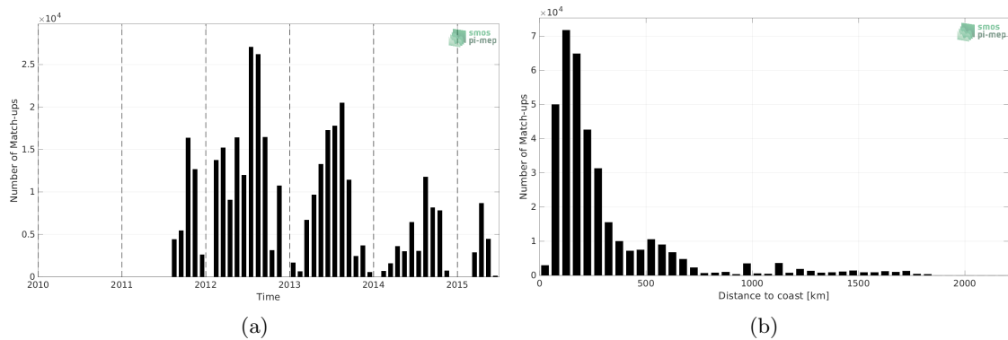
Figure 1: Number of match-ups between TSG (SAMOS) and Aquarius SSS L2 OR v5 (NASA-GSFC) SSS as a function of time (a) and as function of the distance to coast (b) over the Gulf Stream Pi-MEP region and for the full satellite product period.
