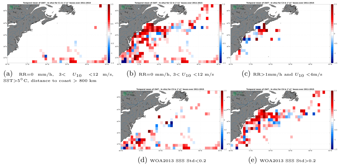
Figure 12: Temporal mean gridded over spatial boxes of size 1^\circ \times 1^\circ of \Delta\text{SSS} (Aquarius SSS L2 OR v5 (NASA-GSFC) - TSG (SAMOS)) for 5 different subdatasets corresponding to:RR=0 mm/h, 3 < U_{10} < 12 m/s, SST >5^\circ\text{C} , distance to coast > 800 km (a), RR=0 mm/h, 3 < U_{10} < 12 m/s (b), RR >1 mm/h and U_{10} < 4 m/s (c), WOA2013 SSS Std <0.2 (d), WOA2013 SSS Std >0.2 (e).
