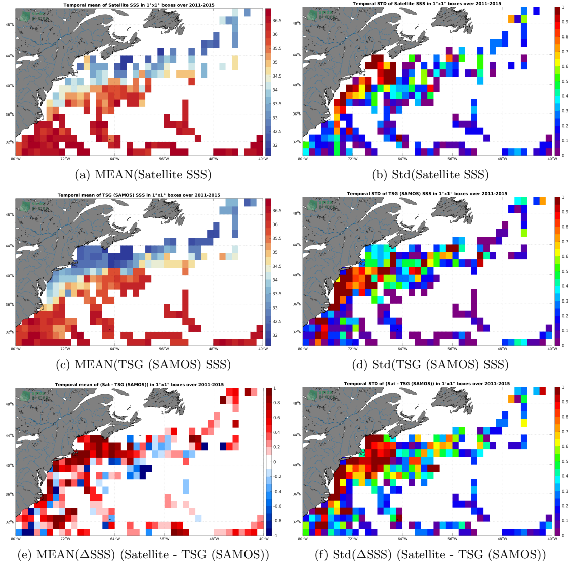
Figure 6: Temporal mean (left) and Std (right) of SSS from Aquarius SSS L2 OR v5 (NASA-GSFC) (top), TSG (SAMOS) (middle), and of \Delta SSS (Satellite - TSG (SAMOS)). Only match-up pairs are used to generate these maps.
