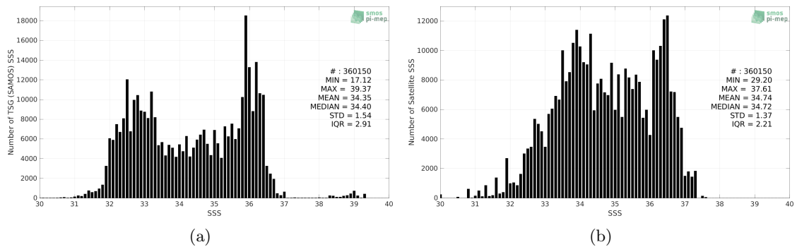
Figure 2: Histograms of SSS from TSG (SAMOS) (a) and Aquarius SSS L2 OR v5 (NASA-GSFC) (b) considering all match-up pairs per bins of 0.1 over the Gulf Stream Pi-MEP region and for the full satellite product period.
