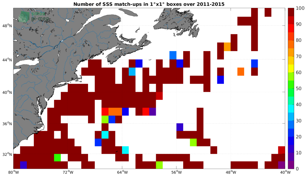
Figure 4: Number of SSS match-ups between TSG (SAMOS) SSS and the Aquarius SSS L2 OR v5 (NASA-GSFC) SSS product for the Gulf Stream Pi-MEP region over 1^\circ \times 1^\circ boxes and for the full satellite product period.
