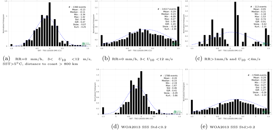
Figure 13: Normalized histogram of \Delta SSS (Aquarius SSS L2 OR v5 (NASA-GSFC) - TSG (LEGOS-DM)) for 5 different subdatasets corresponding to: RR=0 mm/h, 3 < U_{10} < 12 m/s, SST>5°C, distance to coast > 800 km (a), RR=0 mm/h, 3 < U_{10} < 12 m/s (b), RR>1mm/h and U_{10} < 4 m/s (c), WOA2013 SSS Std<0.2 (d), WOA2013 SSS Std>0.2 (e).
