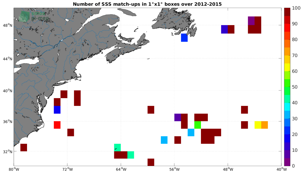
Figure 4: Number of SSS match-ups between TSG (GOSUD-Sailing-ship) SSS and the Aquarius SSS L2 OR v5 (NASA-GSFC) SSS product for the Gulf Stream Pi-MEP region over 1^\circ \times 1^\circ boxes and for the full satellite product period.
