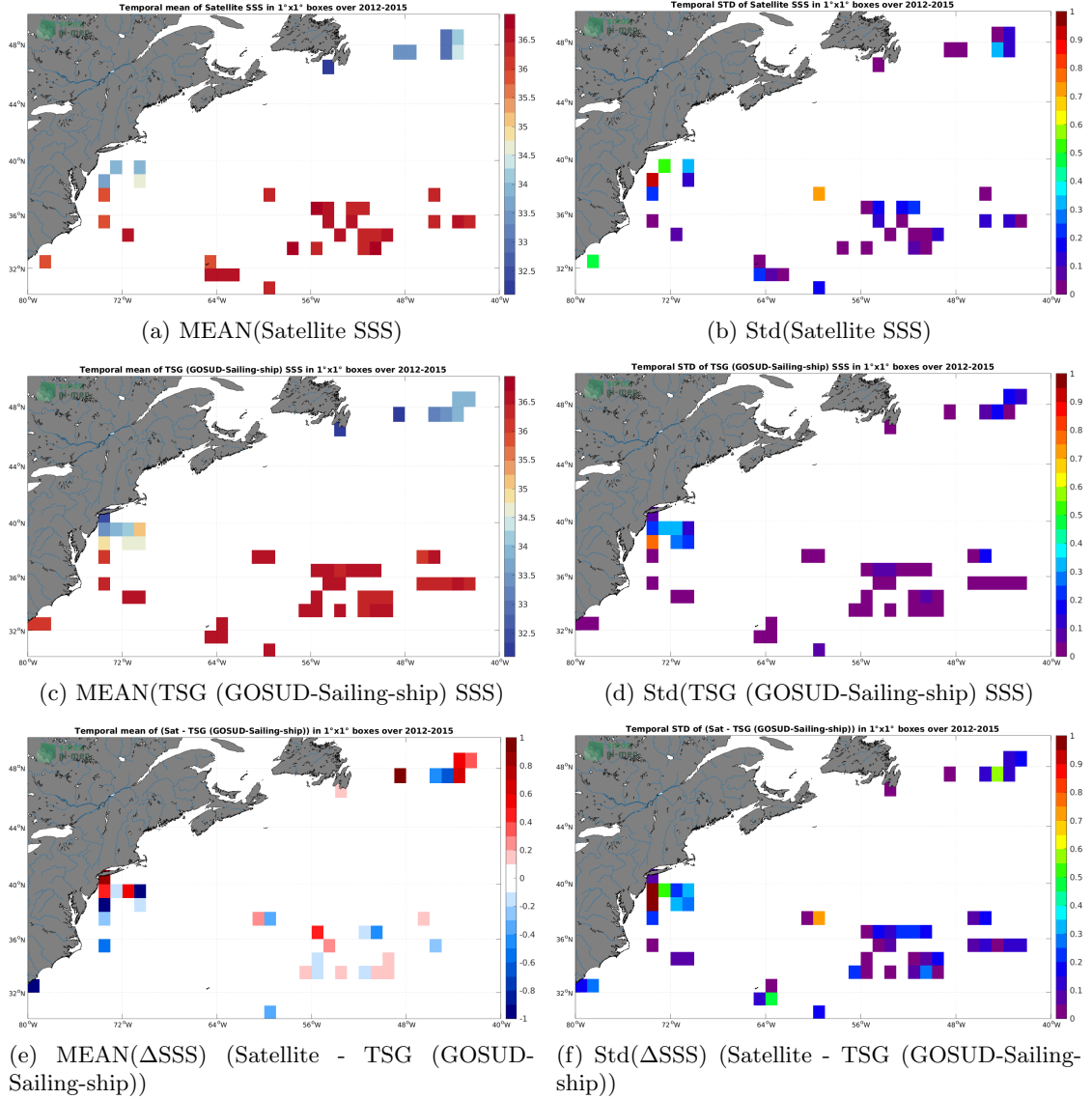
Figure 6: Temporal mean (left) and Std (right) of SSS from Aquarius SSS L2 OR v5 (NASA-GSFC) (top), TSG (GOSUD-Sailing-ship) (middle), and of \Delta SSS (Satellite - TSG (GOSUD-Sailing-ship)). Only match-up pairs are used to generate these maps.
