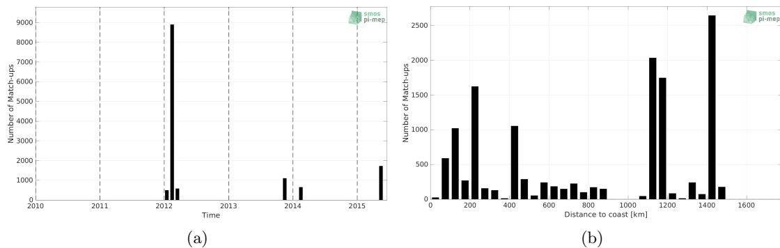
Figure 1: Number of match-ups between TSG (GOSUD-Sailing-ship) and Aquarius SSS L2 OR v5 (NASA-GSFC) SSS as a function of time (a) and as function of the distance to coast (b) over the Gulf Stream Pi-MEP region and for the full satellite product period.
