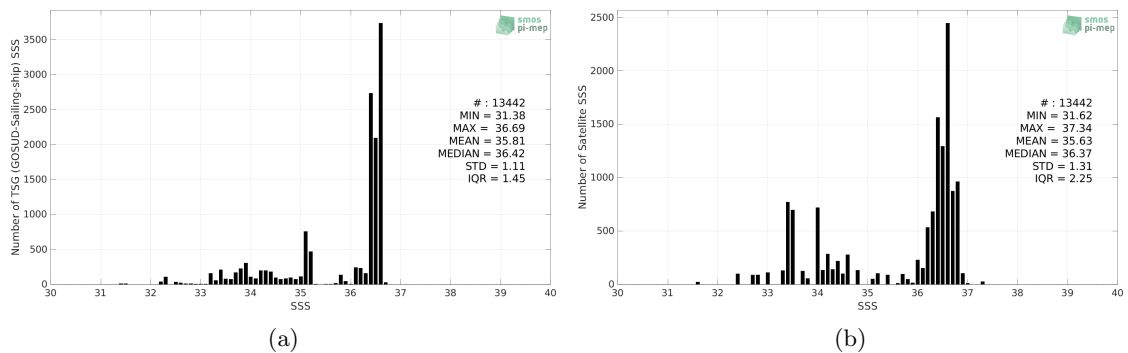
Figure 2: Histograms of SSS from TSG (GOSUD-Sailing-ship) (a) and Aquarius SSS L2 OR v5 (NASA-GSFC) (b) considering all match-up pairs per bins of 0.1 over the Gulf Stream Pi-MEP region and for the full satellite product period.
