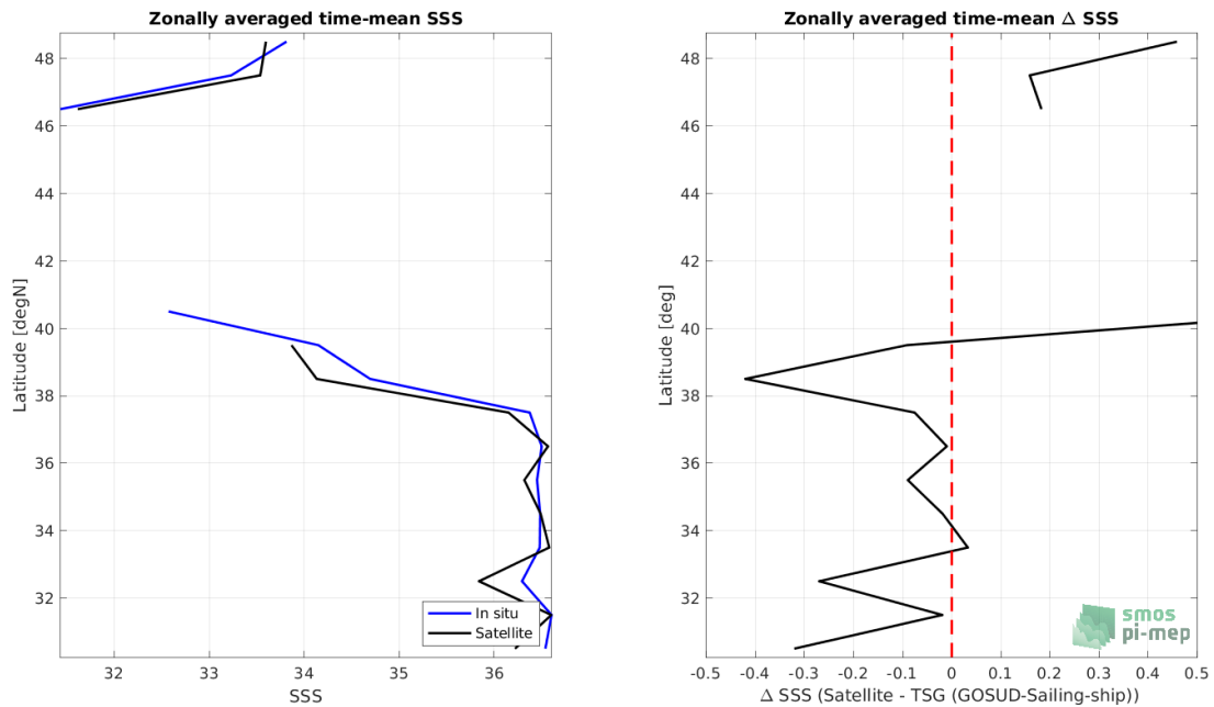
Figure 8: Left panel: Zonal mean SSS from Aquarius SSS L2 OR v5 (NASA-GSFC) satellite product (black) and from TSG (GOSUD-Sailing-ship) (blue). Right panel: Zonal mean of \Delta\text{SSS} (Satellite - TSG (GOSUD-Sailing-ship)) for all the collected Pi-MEP match-up pairs estimated over the full satellite product period.
