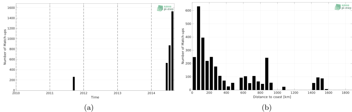
Figure 1: Number of match-ups between TSG (GOSUD-Research-vessel) and Aquarius SSS L2 OR v5 (NASA-GSFC) SSS as a function of time (a) and as function of the distance to coast (b) over the Gulf Stream Pi-MEP region and for the full satellite product period.
