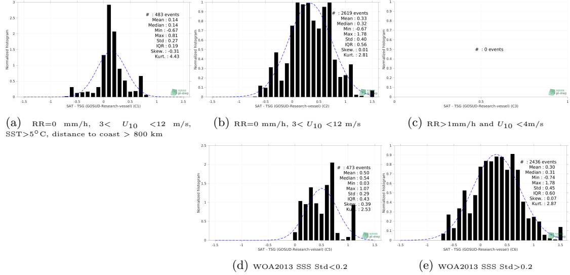
Figure 13: Normalized histogram of \Delta SSS (Aquarius SSS L2 OR v5 (NASA-GSFC) - TSG (GOSUD-Research-vessel)) for 5 different subdatasets corresponding to: RR=0 mm/h, 3 < U_{10} < 12 m/s, SST > 5°C, distance to coast > 800 km (a), RR=0 mm/h, 3 < U_{10} < 12 m/s (b), RR > 1mm/h and U_{10} < 4 m/s (c), WOA2013 SSS Std < 0.2 (d), WOA2013 SSS Std > 0.2 (e).
