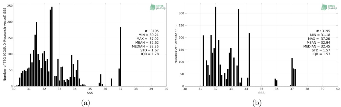
Figure 2: Histograms of SSS from TSG (GOSUD-Research-vessel) (a) and Aquarius SSS L2 OR v5 (NASA-GSFC) (b) considering all match-up pairs per bins of 0.1 over the Gulf Stream Pi-MEP region and for the full satellite product period.
