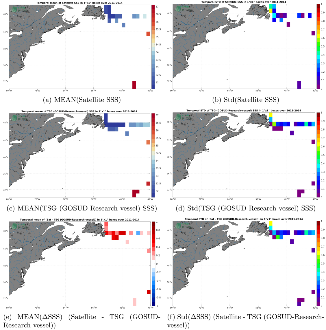
Figure 6: Temporal mean (left) and Std (right) of SSS from Aquarius SSS L2 OR v5 (NASA-GSFC) (top), TSG (GOSUD-Research-vessel) (middle), and of \Delta SSS (Satellite - TSG (GOSUD-Research-vessel)). Only match-up pairs are used to generate these maps.
