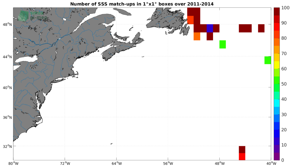
Figure 4: Number of SSS match-ups between TSG (GOSUD-Research-vessel) SSS and the Aquarius SSS L2 OR v5 (NASA-GSFC) SSS product for the Gulf Stream Pi-MEP region over 1^\circ \times 1^\circ boxes and for the full satellite product period.
