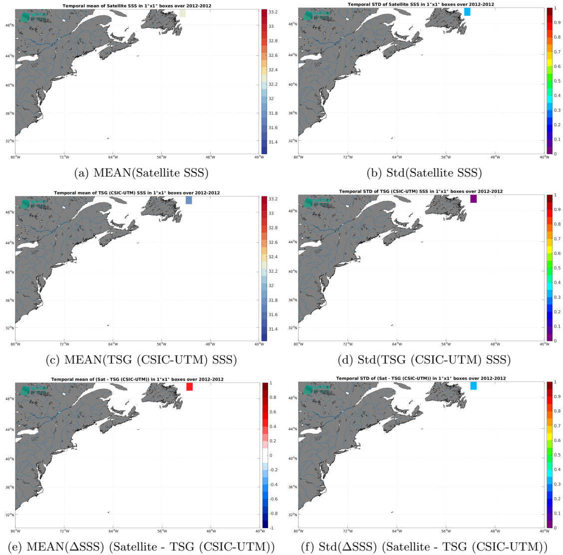
Figure 6: Temporal mean (left) and Std (right) of SSS from Aquarius SSS L2 OR v5 (NASA-GSFC) (top), TSG (CSIC-UTM) (middle), and of \Delta SSS (Satellite - TSG (CSIC-UTM)). Only match-up pairs are used to generate these maps.
