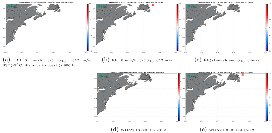
Figure 12: Temporal mean gridded over spatial boxes of size 1^{\circ}\times 1^{\circ} of \Delta\text{SSS} (Aquarius SSS L2 OR v5 (NASA-GSFC) - TSG (CSIC-UTM)) for 5 different subdatasets corresponding to:RR=0 mm/h, 3 < U_{10} < 12 m/s, SST >5^{\circ}\text{C} , distance to coast > 800 km (a), RR=0 mm/h, 3 < U_{10} < 12 m/s (b), RR >1 mm/h and U_{10} < 4 m/s (c), WOA2013 SSS Std <0.2 (d), WOA2013 SSS Std >0.2 (e).
