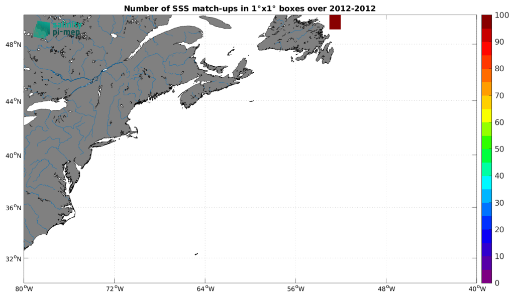
Figure 4: Number of SSS match-ups between TSG (CSIC-UTM) SSS and the Aquarius SSS L2 OR v5 (NASA-GSFC) SSS product for the Gulf Stream Pi-MEP region over 1^\circ \times 1^\circ boxes and for the full satellite product period.
