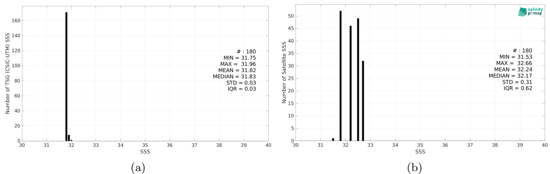
Figure 2: Histograms of SSS from TSG (CSIC-UTM) (a) and Aquarius SSS L2 OR v5 (NASA-GSFC) (b) considering all match-up pairs per bins of 0.1 over the Gulf Stream Pi-MEP region and for the full satellite product period.
