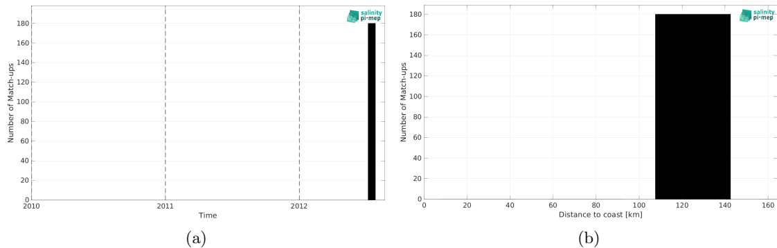
Figure 1: Number of match-ups between TSG (CSIC-UTM) and Aquarius SSS L2 OR v5 (NASA-GSFC) SSS as a function of time (a) and as function of the distance to coast (b) over the Gulf Stream Pi-MEP region and for the full satellite product period.
