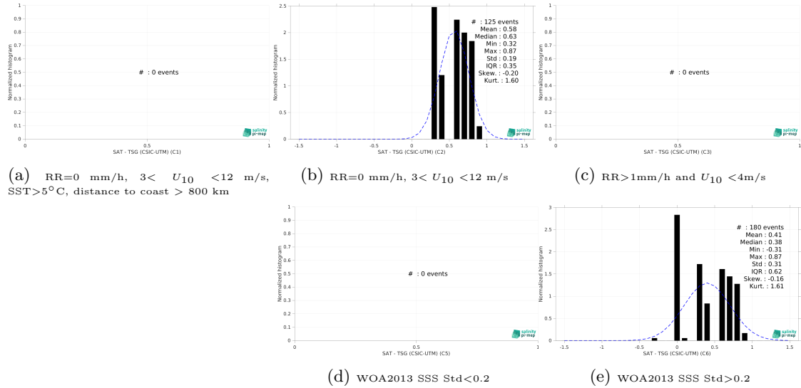
Figure 13: Normalized histogram of \Delta SSS (Aquarius SSS L2 OR v5 (NASA-GSFC) - TSG (CSIC-UTM)) for 5 different subdatasets corresponding to: RR=0 mm/h, 3 < U_{10} < 12 m/s, SST >5^{\circ} C, distance to coast > 800 km (a), RR=0 mm/h, 3 < U_{10} < 12 m/s (b), RR >1 mm/h and U_{10} < 4 m/s (c), WOA2013 SSS Std <0.2 (d), WOA2013 SSS Std >0.2 (e).
