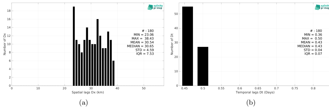
Figure 5: Histograms of the spatial (a) and temporal (b) lags between the location/time of the TSG (CSIC-UTM) measurement and the date of the corresponding Aquarius SSS L2 OR v5 (NASA-GSFC) SSS pixel.
