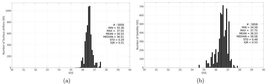
Figure 3: Histograms of SSS from Surface drifters (a) and Aquarius SSS L2 OR v5 (NASA-GSFC) (b) considering all match-up pairs per bins of 0.1 over the Gulf Stream Pi-MEP region and for the full satellite product period.
