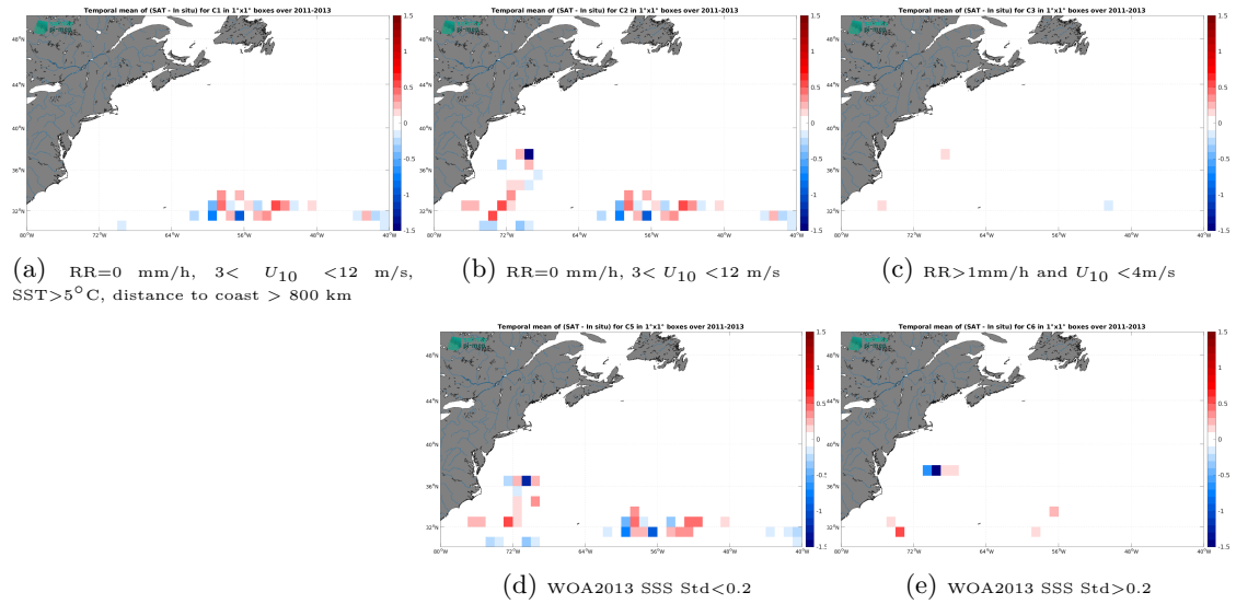
Figure 13: Temporal mean gridded over spatial boxes of size 1^\circ \times 1^\circ of \Delta SSS (Aquarius SSS L2 OR v5 (NASA-GSFC) - Surface drifters) for 5 different subdatasets corresponding to:RR=0 mm/h, 3 < U_{10} < 12 m/s, SST >5^\circ C, distance to coast > 800 km (a), RR=0 mm/h, 3 < U_{10} < 12 m/s (b), RR >1 mm/h and U_{10} < 4 m/s (c), WOA2013 SSS Std <0.2 (d), WOA2013 SSS Std >0.2 (e).
