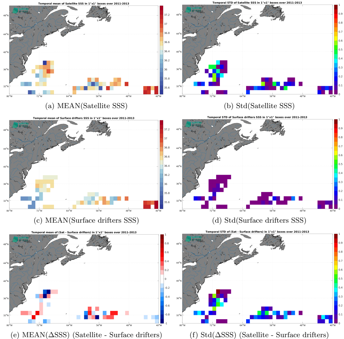
Figure 6: Temporal mean (left) and Std (right) of SSS from Aquarius SSS L2 OR v5 (NASA-GSFC) (top), Surface drifters (middle), and of \Delta SSS (Satellite - Surface drifters). Only match-up pairs are used to generate these maps.
