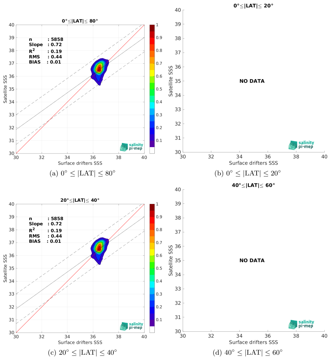
Figure 9: Contour maps of the concentration of Aquarius SSS L2 OR v5 (NASA-GSFC) SSS (y-axis) versus Surface drifters SSS (x-axis) at match-up pairs for different latitude bands. For each plot, the red line shows x=y . The black thin and dashed lines indicate a linear fit through the data cloud and the \pm 95\% confidence levels, respectively. The number match-up pairs n , the slope and R^2 coefficient of the linear fit, the root mean square (RMS) and the mean bias between satellite and in situ data are indicated for each latitude band in each plots.
