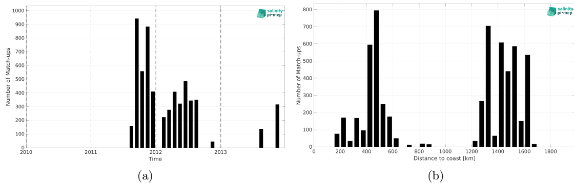
Figure 2: Number of match-ups between Surface drifters and Aquarius SSS L2 OR v5 (NASA-GSFC) SSS as a function of time (a) and as function of the distance to coast (b) over the Gulf Stream Pi-MEP region and for the full satellite product period.
