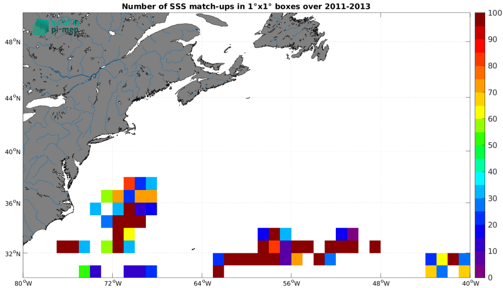
Figure 4: Number of SSS match-ups between Surface drifters SSS and the Aquarius SSS L2 OR v5 (NASA-GSFC) SSS product for the Gulf Stream Pi-MEP region over 1^\circ \times 1^\circ boxes and for the full satellite product period.
