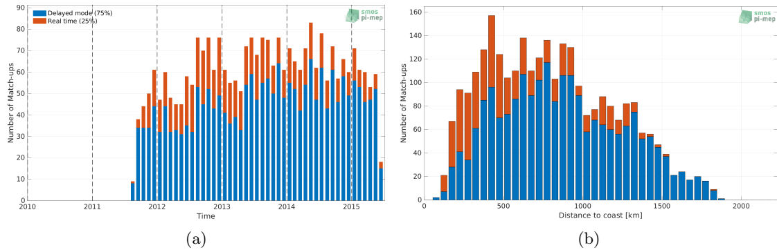
Figure 1: Number of match-ups between Argo and Aquarius SSS L2 OR v5 (NASA-GSFC) SSS as a function of time (a) and as function of the distance to coast (b) over the Gulf Stream Pi-MEP region and for the full satellite product period.
