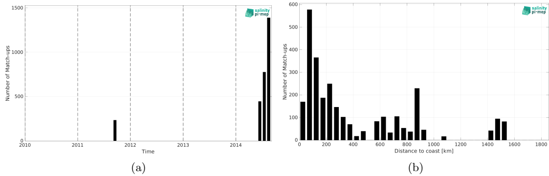
Figure 2: Number of match-ups between TSG (GOSUD-Research-vessel) and Aquarius SSS L2 CAP v5 (JPL) SSS as a function of time (a) and as function of the distance to coast (b) over the Gulf Stream Pi-MEP region and for the full satellite product period.
