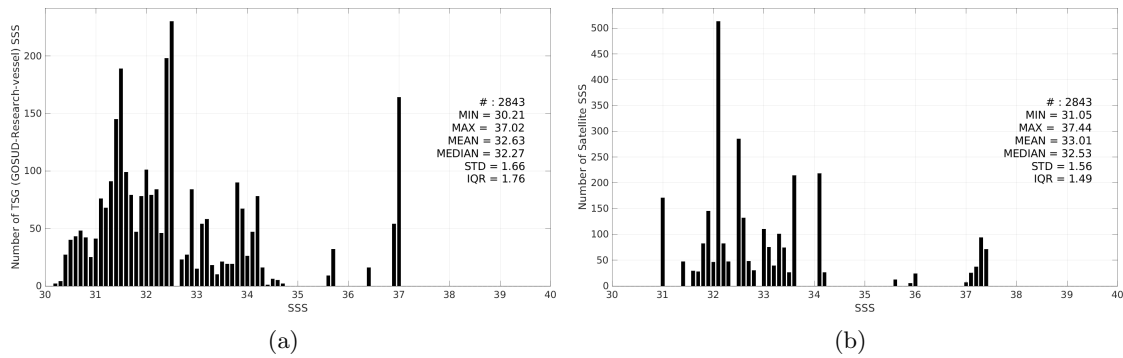
Figure 3: Histograms of SSS from TSG (GOSUD-Research-vessel) (a) and Aquarius SSS L2 CAP v5 (JPL) (b) considering all match-up pairs per bins of 0.1 over the Gulf Stream Pi-MEP region and for the full satellite product period.
