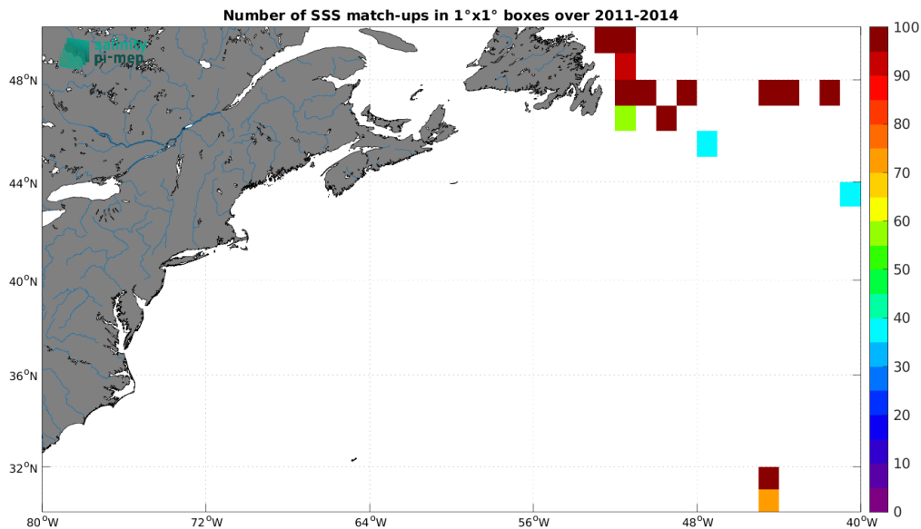
Figure 5: Number of SSS match-ups between TSG (GOSUD-Research-vessel) SSS and the Aquarius SSS L2 CAP v5 (JPL) SSS product for the Gulf Stream Pi-MEP region over 1^\circ \times 1^\circ boxes and for the full satellite product period.
