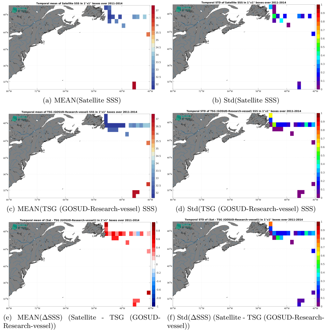
Figure 7: Temporal mean (left) and Std (right) of SSS from Aquarius SSS L2 CAP v5 (JPL) (top), TSG (GOSUD-Research-vessel) (middle), and of \Delta SSS (Satellite - TSG (GOSUD-Research-vessel)). Only match-up pairs are used to generate these maps.
