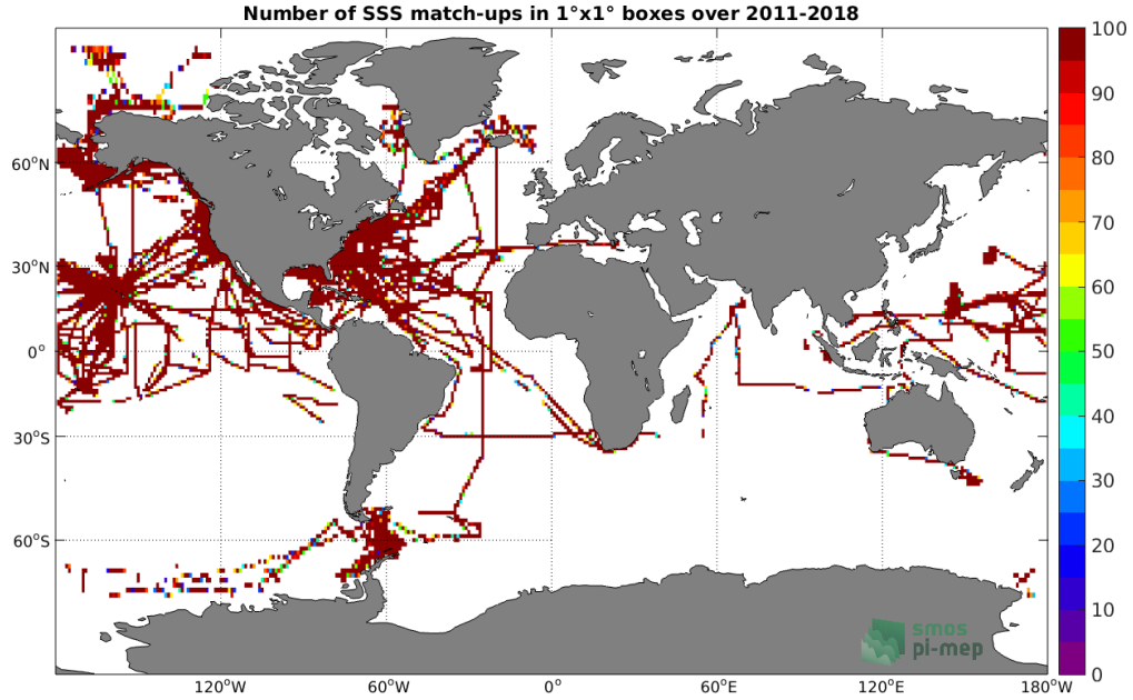
Figure 4: Number of SSS match-ups between TSG (SAMOS) SSS and the SMOS and SMAP SSS L4 OI v1 - 7 Days (LOPS) SSS product for the Global Ocean Pi-MEP region over 1^\circ \times 1^\circ boxes and for the full satellite product period.
