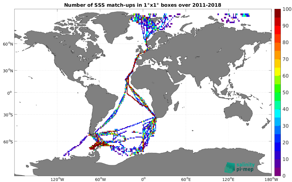
Figure 4: Number of SSS match-ups between TSG (Polarstern) SSS and the SMOS and SMAP SSS L4 OI v1 - 7 Days (LOPS) SSS product for the Global Ocean Pi-MEP region over 1^\circ \times 1^\circ boxes and for the full satellite product period.
