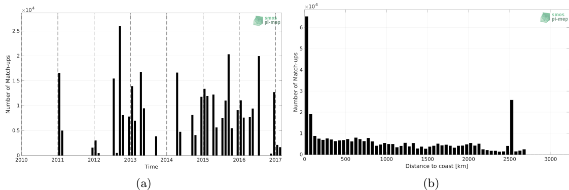
Figure 1: Number of match-ups between TSG (NCEI-0170743) and SMOS and SMAP SSS L4 OI v1 - 7 Days (LOPS) SSS as a function of time (a) and as function of the distance to coast (b) over the Global Ocean Pi-MEP region and for the full satellite product period.
