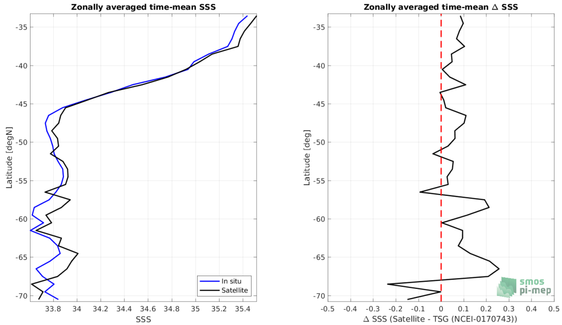
Figure 8: Left panel: Zonal mean SSS from SMOS and SMAP SSS L4 OI v1 - 7 Days (LOPS) satellite product (black) and from TSG (NCEI-0170743) (blue). Right panel: Zonal mean of \Delta SSS (Satellite - TSG (NCEI-0170743)) for all the collected Pi-MEP match-up pairs estimated over the full satellite product period.
