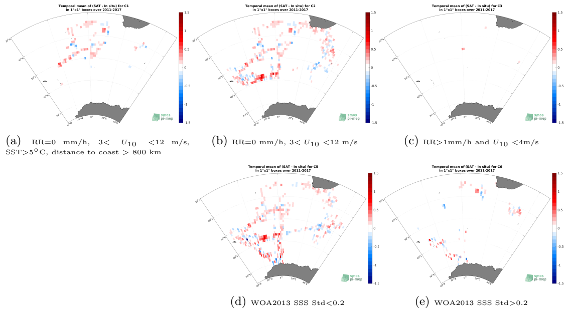
Figure 12: Temporal mean gridded over spatial boxes of size 1^\circ \times 1^\circ of \Delta SSS (SMOS and SMAP SSS L4 OI v1 - 7 Days (LOPS) - TSG (NCEI-0170743)) for 5 different subdatasets corresponding to:RR=0 mm/h, 3 < U_{10} < 12 m/s, SST > 5^\circ\text{C} , distance to coast > 800 km (a), RR=0 mm/h, 3 < U_{10} < 12 m/s (b), RR > 1 mm/h and U_{10} < 4 m/s (c), WOA2013 SSS Std < 0.2 (d), WOA2013 SSS Std > 0.2 (e).
