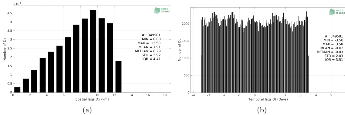
Figure 5: Histograms of the spatial (a) and temporal (b) lags between the location/time of the TSG (NCEI-0170743) measurement and the date of the corresponding SMOS and SMAP SSS L4 OI v1 - 7 Days (LOPS) SSS pixel.
