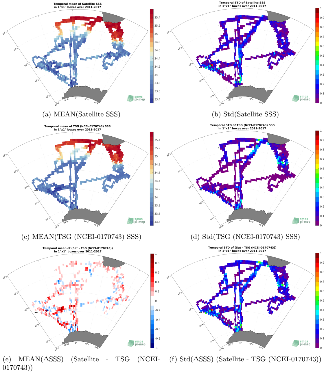
Figure 6: Temporal mean (left) and Std (right) of SSS from SMOS and SMAP SSS L4 OI v1 - 7 Days (LOPS) (top), TSG (NCEI-0170743) (middle), and of \Delta SSS (Satellite - TSG (NCEI-0170743)). Only match-up pairs are used to generate these maps.
