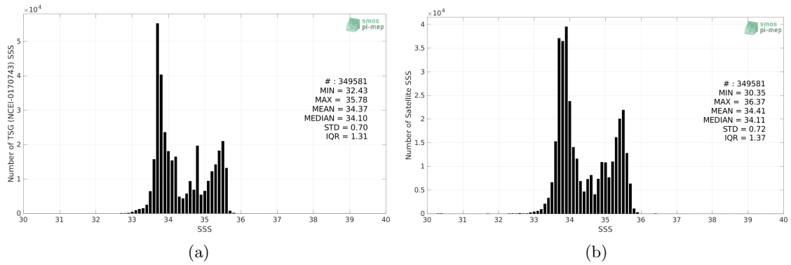
Figure 2: Histograms of SSS from TSG (NCEI-0170743) (a) and SMOS and SMAP SSS L4 OI v1 - 7 Days (LOPS) (b) considering all match-up pairs per bins of 0.1 over the Global Ocean Pi-MEP region and for the full satellite product period.
