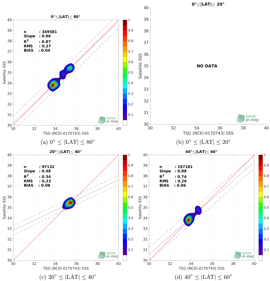
Figure 9: Contour maps of the concentration of SMOS and SMAP SSS L4 OI v1 - 7 Days (LOPS) SSS (y-axis) versus TSG (NCEI-0170743) SSS (x-axis) at match-up pairs for different latitude bands. For each plot, the red line shows x=y . The black thin and dashed lines indicate a linear fit through the data cloud and the \pm 95\% confidence levels, respectively. The number match-up pairs n , the slope and R^2 coefficient of the linear fit, the root mean square (RMS) and the mean bias between satellite and in situ data are indicated for each latitude band in each plots.
