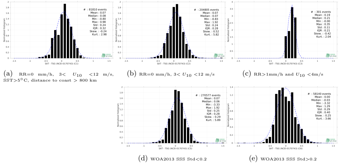
Figure 13: Normalized histogram of \Delta\text{SSS} (SMOS and SMAP SSS L4 OI v1 - 7 Days (LOPS) - TSG (NCEI-0170743)) for 5 different subdatasets corresponding to: RR=0 mm/h, 3 < U_{10} < 12 m/s, SST >5^{\circ}\text{C} , distance to coast > 800 km (a), RR=0 mm/h, 3 < U_{10} < 12 m/s (b), RR >1 mm/h and U_{10} < 4 m/s (c), WOA2013 SSS Std <0.2 (d), WOA2013 SSS Std >0.2 (e).
