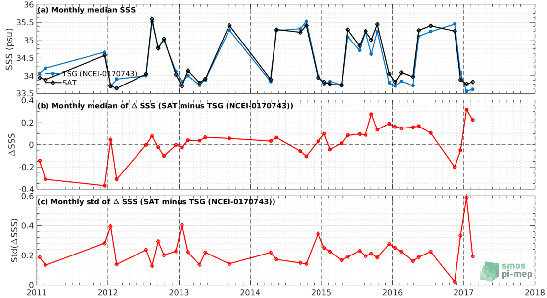
Figure 7: Time series of the monthly median SSS (top), median of \Delta\text{SSS} (Satellite - TSG (NCEI-0170743)) and Std of \Delta\text{SSS} (Satellite - TSG (NCEI-0170743)) over the Global Ocean Pi-MEP region considering all match-ups collected by the Pi-MEP.
