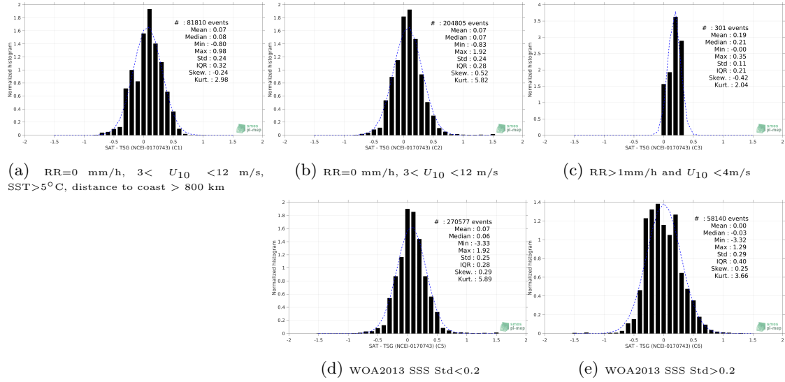
Figure 13: Normalized histogram of \Delta SSS (SMOS and SMAP SSS L4 OI v1 - 7 Days (LOPS) - TSG (NCEI-0170743)) for 5 different subdatasets corresponding to: RR=0 mm/h, 3 < U_{10} < 12 m/s, SST>5°C, distance to coast > 800 km (a), RR=0 mm/h, 3 < U_{10} < 12 m/s (b), RR>1mm/h and U_{10} < 4 m/s (c), WOA2013 SSS Std<0.2 (d), WOA2013 SSS Std>0.2 (e).
