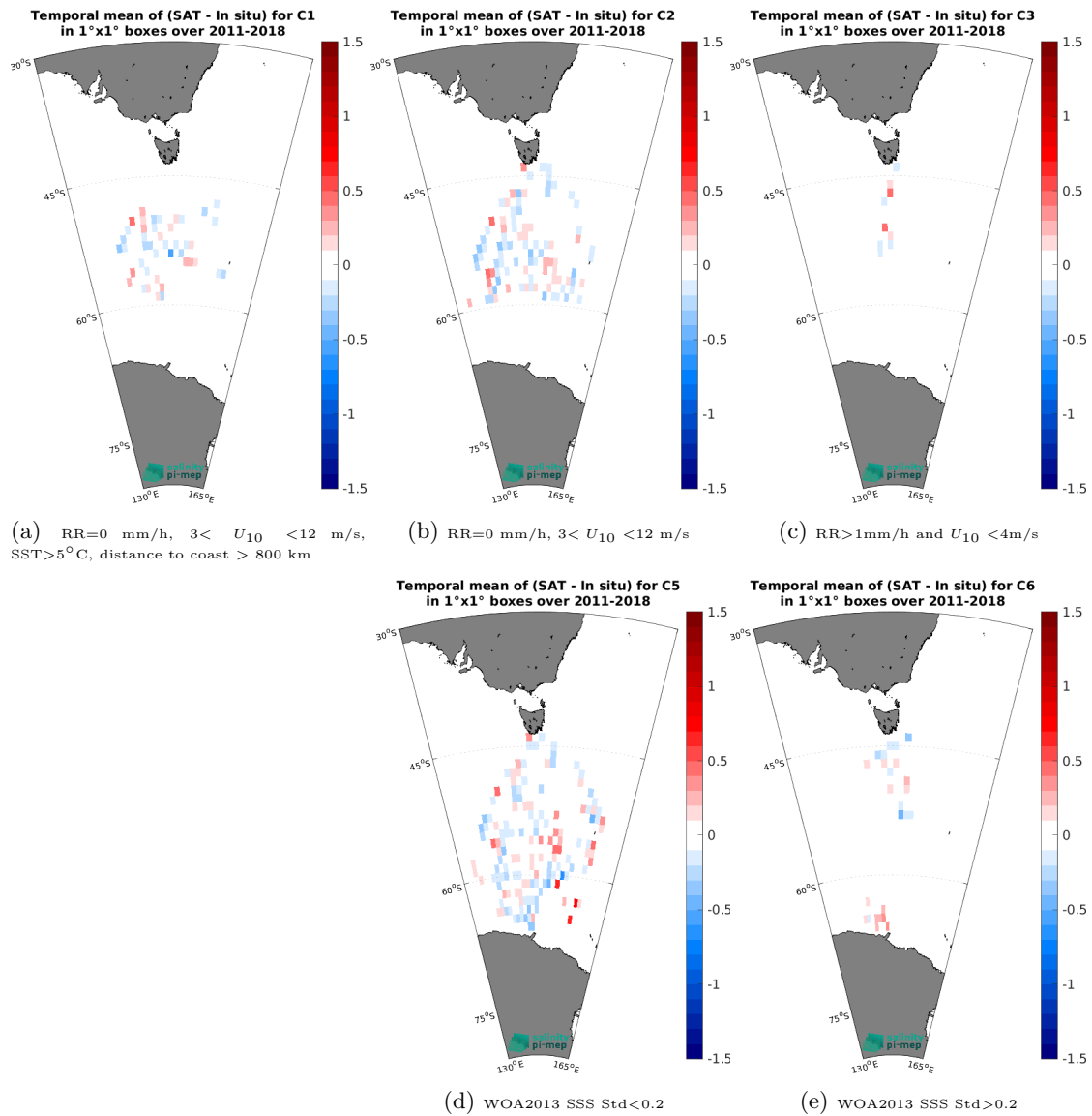
Figure 12: Temporal mean gridded over spatial boxes of size 1^\circ \times 1^\circ of \Delta\text{SSS} (SMOS and SMAP SSS L4 OI v1 - 7 Days (LOPS) - TSG (LEGOS-Survostral)) for 5 different subdatasets corresponding to: RR=0 mm/h, 3 < U_{10} < 12 m/s, SST > 5^\circ\text{C} , distance to coast > 800 km (a), RR=0 mm/h, 3 < U_{10} < 12 m/s (b), RR > 1 mm/h and U_{10} < 4 m/s (c), WOA2013 SSS Std < 0.2 (d), WOA2013 SSS Std > 0.2 (e).
