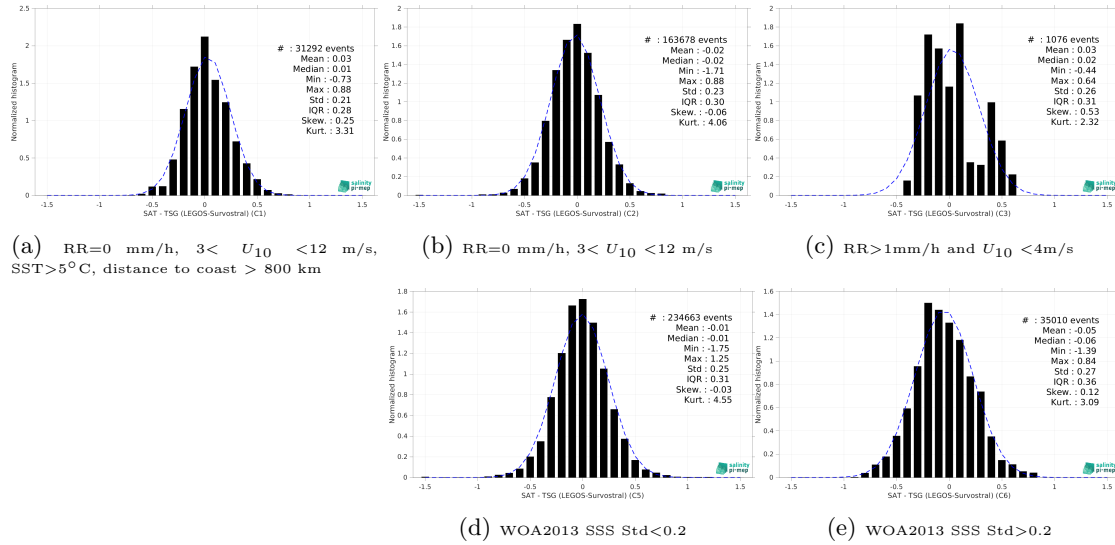
Figure 13: Normalized histogram of \Delta SSS (SMOS and SMAP SSS L4 OI v1 - 7 Days (LOPS) - TSG (LEGOS-Survostral)) for 5 different subdatasets corresponding to: RR=0 mm/h, 3 < U_{10} < 12 m/s, SST>5°C, distance to coast > 800 km (a), RR=0 mm/h, 3 < U_{10} < 12 m/s (b), RR>1mm/h and U_{10} < 4 m/s (c), WOA2013 SSS Std<0.2 (d), WOA2013 SSS Std>0.2 (e).
