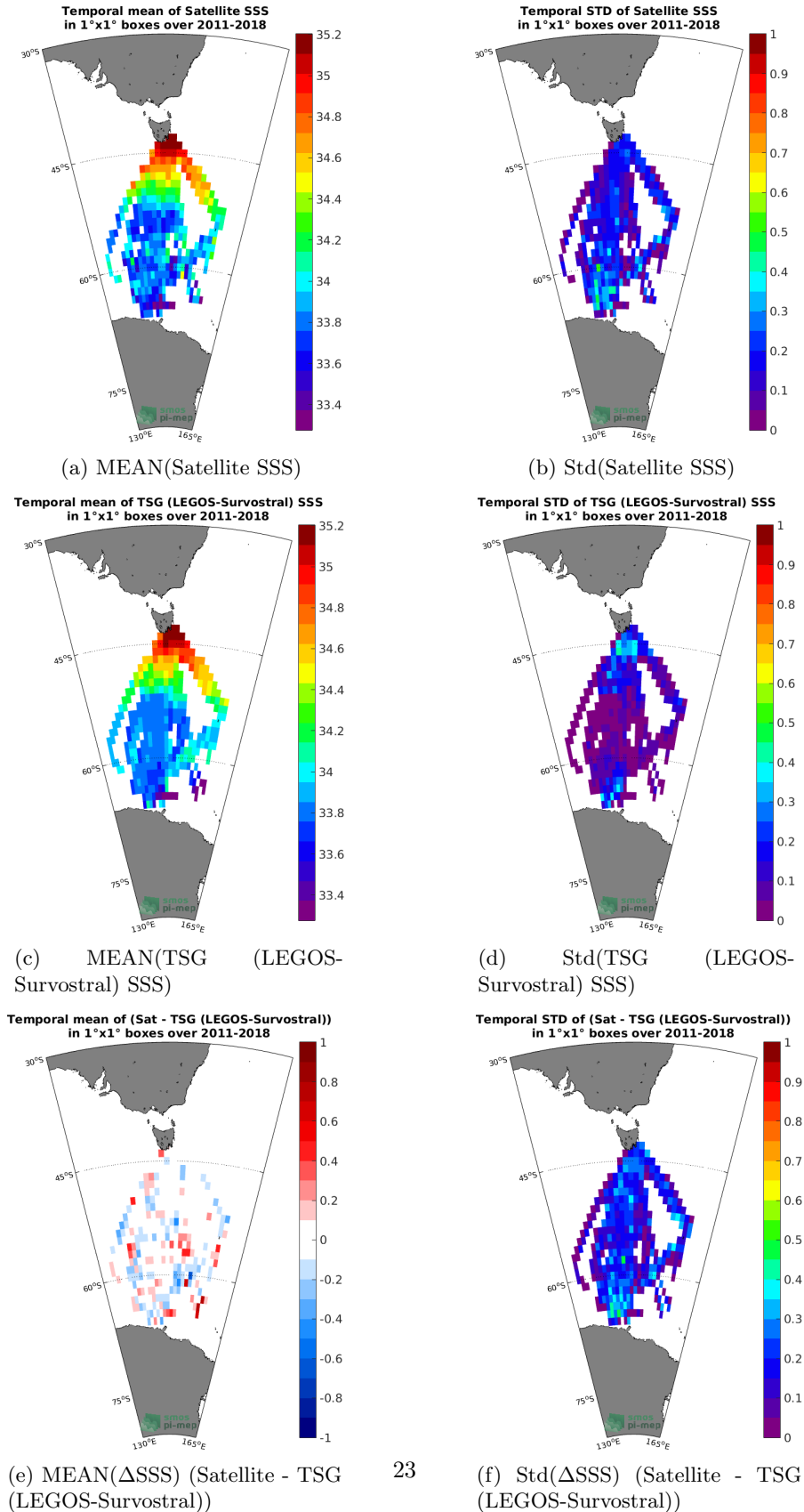
Figure 6: Temporal mean (left) and Std (right) of SSS from SMOS and SMAP SSS L4 OI v1 - 7 Days (LOPS) (top), TSG (LEGOS-Survostral) (middle), and of ΔSSS (Satellite - TSG (LEGOS-Survostral)). Only match-up pairs are used to generate these maps.
