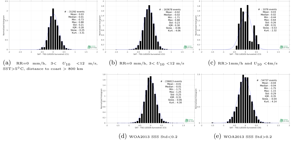
Figure 13: Normalized histogram of \Delta SSS (SMOS and SMAP SSS L4 OI v1 - 7 Days (LOPS) - TSG (LEGOS-Survostral)) for 5 different subdatasets corresponding to: RR=0 mm/h, 3 < U_{10} < 12 m/s, SST>5°C, distance to coast > 800 km (a), RR=0 mm/h, 3 < U_{10} < 12 m/s (b), RR>1mm/h and U_{10} < 4 m/s (c), WOA2013 SSS Std<0.2 (d), WOA2013 SSS Std>0.2 (e).
