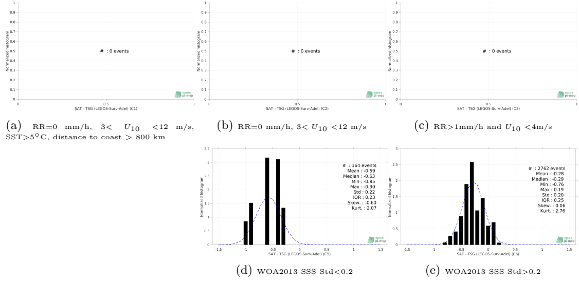
Figure 13: Normalized histogram of \Delta SSS (SMOS and SMAP SSS L4 OI v1 - 7 Days (LOPS) - TSG (LEGOS-Surv-Adel)) for 5 different subdatasets corresponding to: RR=0 mm/h, 3 < U_{10} < 12 m/s, SST > 5°C, distance to coast > 800 km (a), RR=0 mm/h, 3 < U_{10} < 12 m/s (b), RR > 1mm/h and U_{10} < 4 m/s (c), WOA2013 SSS Std < 0.2 (d), WOA2013 SSS Std > 0.2 (e).
