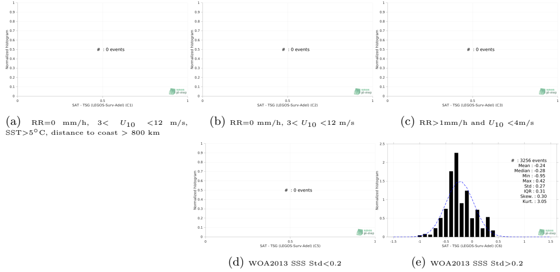
Figure 13: Normalized histogram of \Delta\text{SSS} (SMOS and SMAP SSS L4 OI v1 - 7 Days (LOPS) - TSG (LEGOS-Surv-Adel)) for 5 different subdatasets corresponding to: RR=0 mm/h, 3 < U_{10} < 12 m/s, SST > 5^\circ\text{C} , distance to coast > 800 km (a), RR=0 mm/h, 3 < U_{10} < 12 m/s (b), RR > 1\text{mm/h} and U_{10} < 4\text{m/s} (c), WOA2013 SSS Std < 0.2 (d), WOA2013 SSS Std > 0.2 (e).
