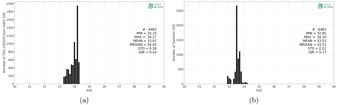
Figure 2: Histograms of SSS from TSG (LEGOS-Surv-Adel) (a) and SMOS and SMAP SSS L4 OI v1 - 7 Days (LOPS) (b) considering all match-up pairs per bins of 0.1 over the Global Ocean Pi-MEP region and for the full satellite product period.
