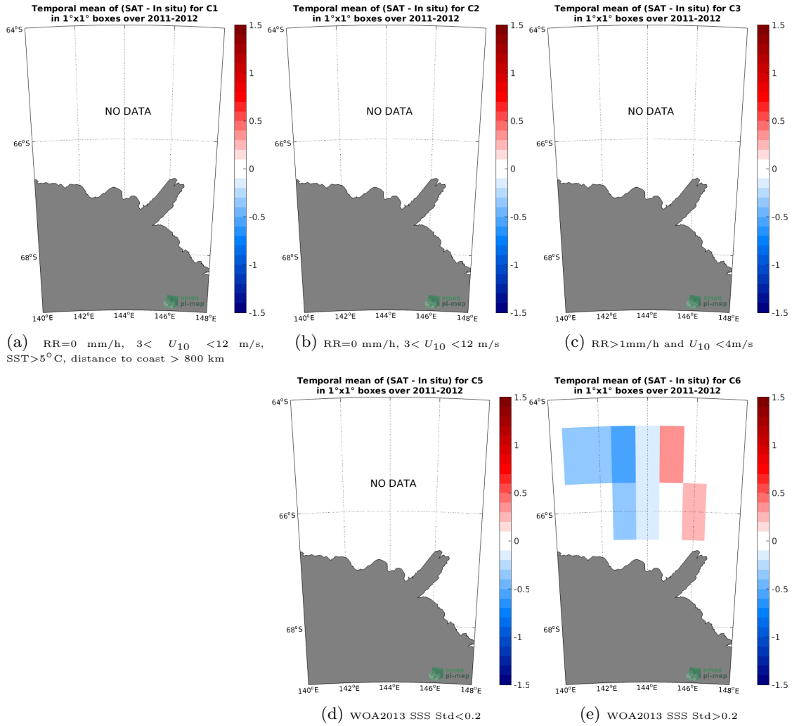
Figure 12: Temporal mean gridded over spatial boxes of size 1^\circ \times 1^\circ of \Delta SSS (SMOS and SMAP SSS L4 OI v1 - 7 Days (LOPS) - TSG (LEGOS-Surv-Adel)) for 5 different subdatasets corresponding to: RR=0 mm/h, 3 < U_{10} < 12 m/s, SST > 5°C, distance to coast > 800 km (a), RR=0 mm/h, 3 < U_{10} < 12 m/s (b), RR > 1mm/h and U_{10} < 4 m/s (c), WOA2013 SSS Std < 0.2 (d), WOA2013 SSS Std > 0.2 (e).
