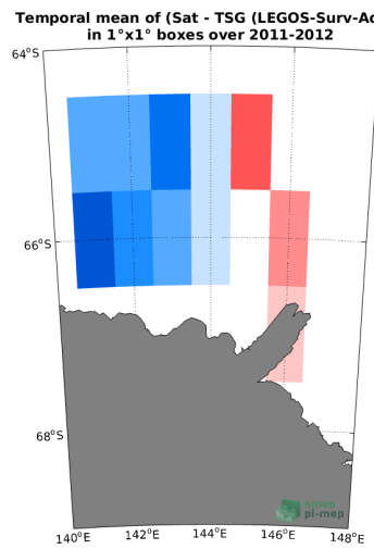
(e) MEAN( \Delta SSS) (Satellite - TSG (LEGOS-Surv-Adel))
