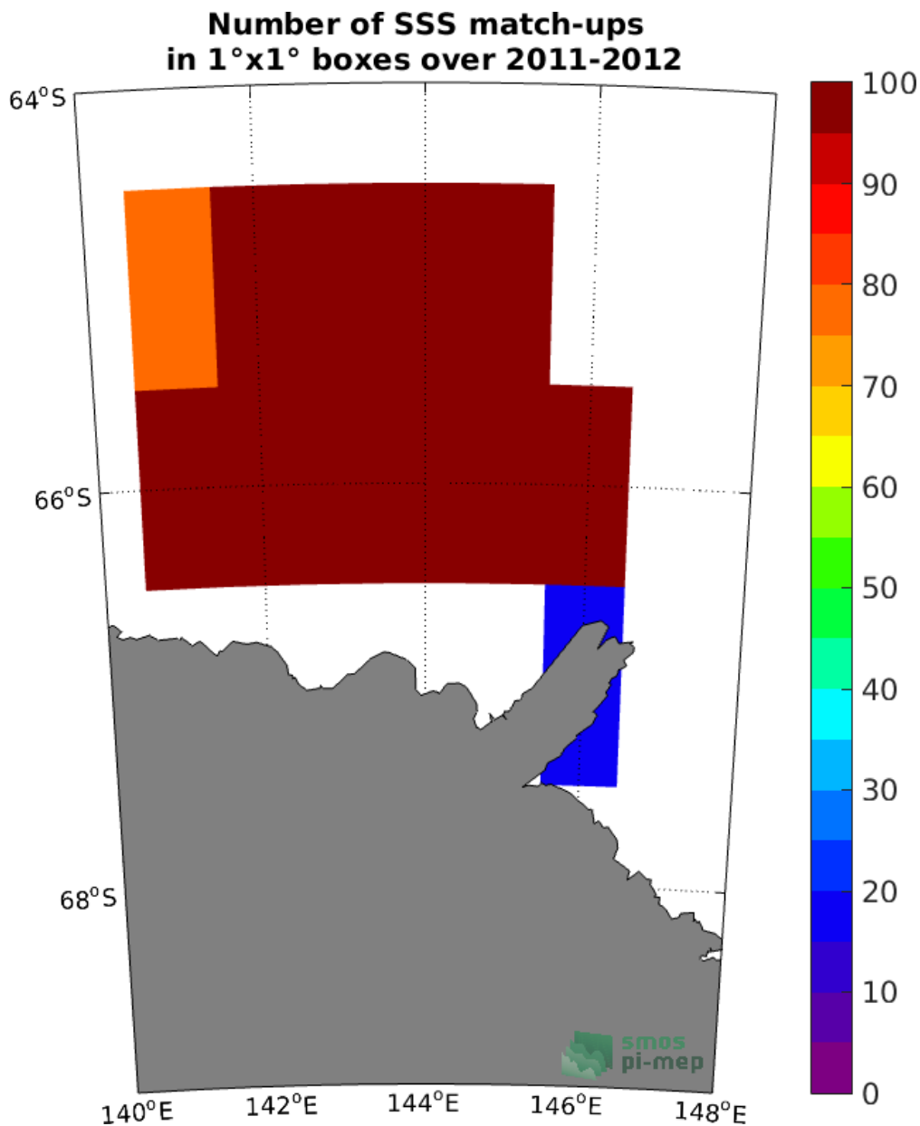
Figure 4: Number of SSS match-ups between TSG (LEGOS-Surv-Adel) SSS and the SMOS and SMAP SSS L4 OI v1 - 7 Days (LOPS) SSS product for the Global Ocean Pi-MEP region over 1^\circ \times 1^\circ boxes and for the full satellite product period.
