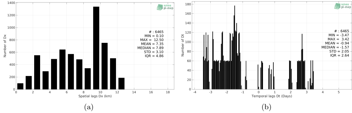
Figure 5: Histograms of the spatial (a) and temporal (b) lags between the location/time of the TSG (LEGOS-Surv-Adel) measurement and the date of the corresponding SMOS and SMAP SSS L4 OI v1 - 7 Days (LOPS) SSS pixel.
