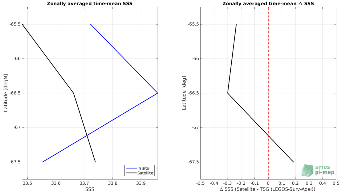
Figure 8: Left panel: Zonal mean SSS from SMOS and SMAP SSS L4 OI v1 - 7 Days (LOPS) satellite product (black) and from TSG (LEGOS-Surv-Adel) (blue). Right panel: Zonal mean of \Delta SSS (Satellite - TSG (LEGOS-Surv-Adel)) for all the collected Pi-MEP match-up pairs estimated over the full satellite product period.
