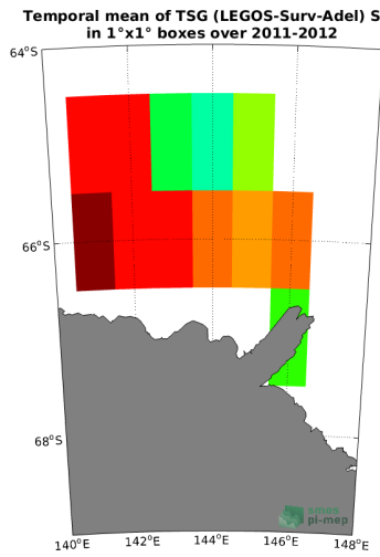
(c) MEAN(TSG (LEGOS-Surv-Adel) SSS)
