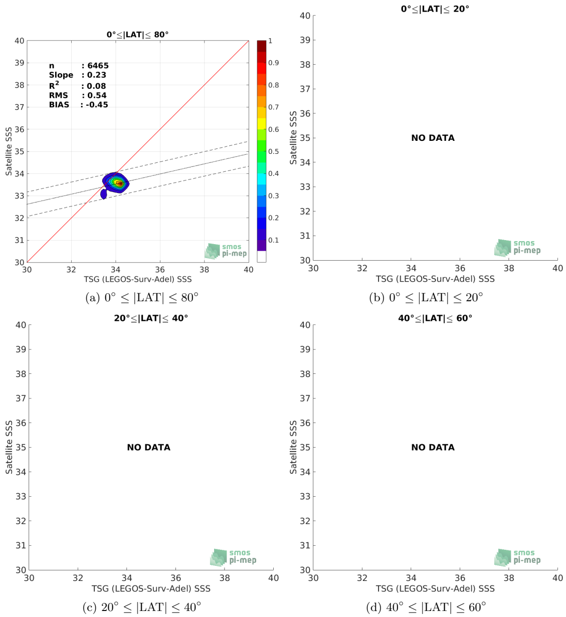
Figure 9: Contour maps of the concentration of SMOS and SMAP SSS L4 OI v1 - 7 Days (LOPS) SSS (y-axis) versus TSG (LEGOS-Surv-Adel) SSS (x-axis) at match-up pairs for different latitude bands. For each plot, the red line shows x=y . The black thin and dashed lines indicate a linear fit through the data cloud and the \pm 95\% confidence levels, respectively. The number match-up pairs n , the slope and R^2 coefficient of the linear fit, the root mean square (RMS) and the mean bias between satellite and in situ data are indicated for each latitude band in each plots.
