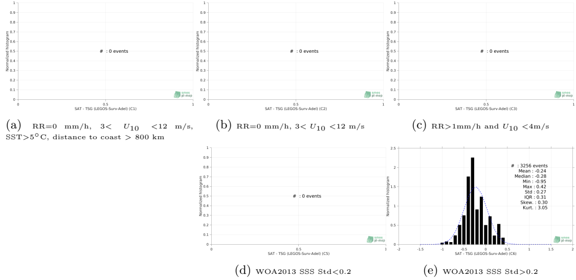
Figure 13: Normalized histogram of \Delta SSS (SMOS and SMAP SSS L4 OI v1 - 7 Days (LOPS) - TSG (LEGOS-Surv-Adel)) for 5 different subdatasets corresponding to: RR=0 mm/h, 3 < U_{10} < 12 m/s, SST>5°C, distance to coast > 800 km (a), RR=0 mm/h, 3 < U_{10} < 12 m/s (b), RR>1mm/h and U_{10} < 4 m/s (c), WOA2013 SSS Std<0.2 (d), WOA2013 SSS Std>0.2 (e).
