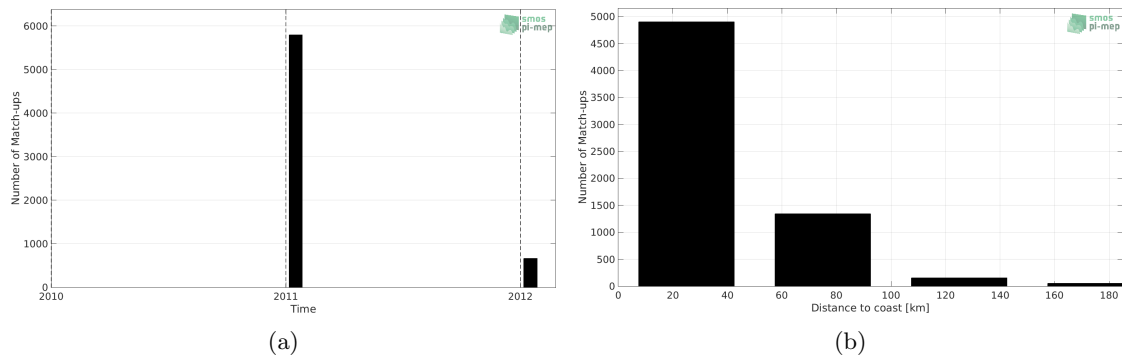
Figure 1: Number of match-ups between TSG (LEGOS-Surv-Adel) and SMOS and SMAP SSS L4 OI v1 - 7 Days (LOPS) SSS as a function of time (a) and as function of the distance to coast (b) over the Global Ocean Pi-MEP region and for the full satellite product period.
