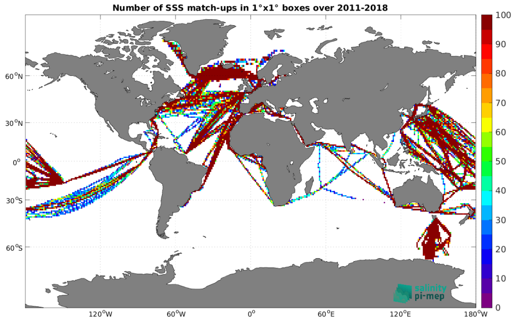
Figure 4: Number of SSS match-ups between TSG (LEGOS-DM) SSS and the SMOS and SMAP SSS L4 OI v1 - 7 Days (LOPS) SSS product for the Global Ocean Pi-MEP region over 1^\circ \times 1^\circ boxes and for the full satellite product period.
