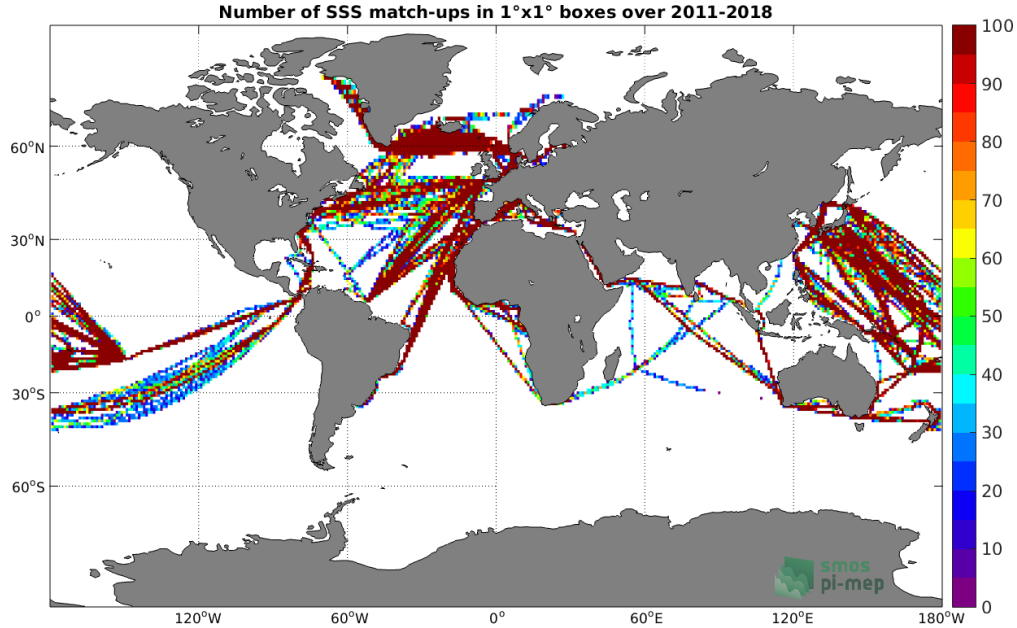
Figure 4: Number of SSS match-ups between TSG (LEGOS-DM) SSS and the SMOS and SMAP SSS L4 OI v1 - 7 Days (LOPS) SSS product for the Global Ocean Pi-MEP region over 1^\circ \times 1^\circ boxes and for the full satellite product period.
