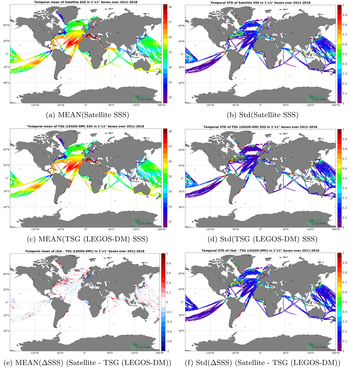
Figure 6: Temporal mean (left) and Std (right) of SSS from SMOS and SMAP SSS L4 OI v1 - 7 Days (LOPS) (top), TSG (LEGOS-DM) (middle), and of \Delta SSS (Satellite - TSG (LEGOS-DM)). Only match-up pairs are used to generate these maps.
