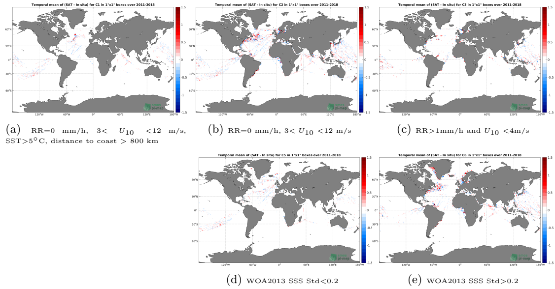
Figure 12: Temporal mean gridded over spatial boxes of size 1^\circ \times 1^\circ of \Delta SSS (SMOS and SMAP SSS L4 OI v1 - 7 Days (LOPS) - TSG (LEGOS-DM)) for 5 different subdatasets corresponding to: RR=0 mm/h, 3 < U_{10} < 12 m/s, SST > 5^\circ\text{C} , distance to coast > 800 km (a), RR=0 mm/h, 3 < U_{10} < 12 m/s (b), RR > 1 mm/h and U_{10} < 4 m/s (c), WOA2013 SSS Std < 0.2 (d), WOA2013 SSS Std > 0.2 (e).
