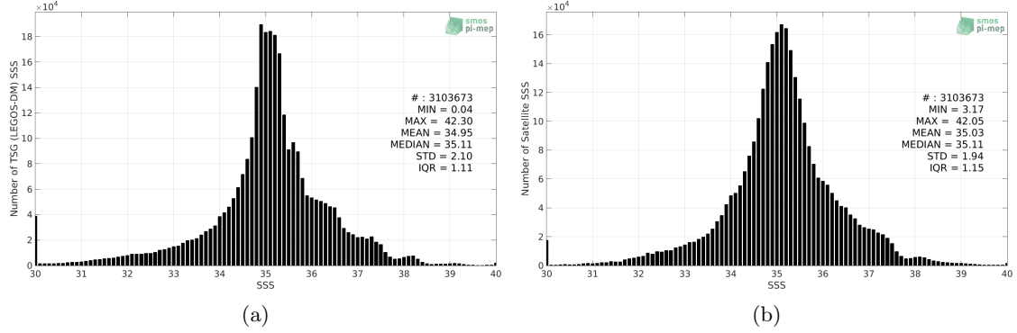
Figure 2: Histograms of SSS from TSG (LEGOS-DM) (a) and SMOS and SMAP SSS L4 OI v1 - 7 Days (LOPS) (b) considering all match-up pairs per bins of 0.1 over the Global Ocean Pi-MEP region and for the full satellite product period.
