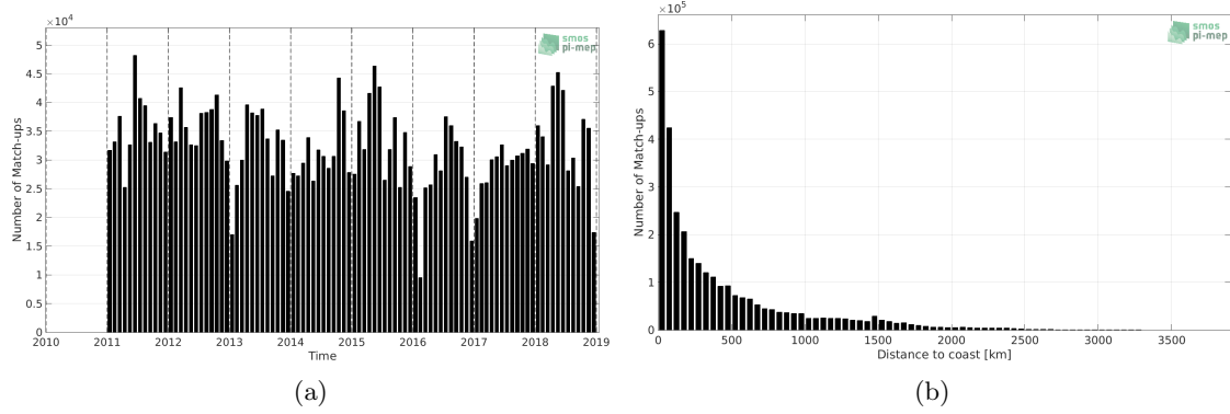
Figure 1: Number of match-ups between TSG (LEGOS-DM) and SMOS and SMAP SSS L4 OI v1 - 7 Days (LOPS) SSS as a function of time (a) and as function of the distance to coast (b) over the Global Ocean Pi-MEP region and for the full satellite product period.
