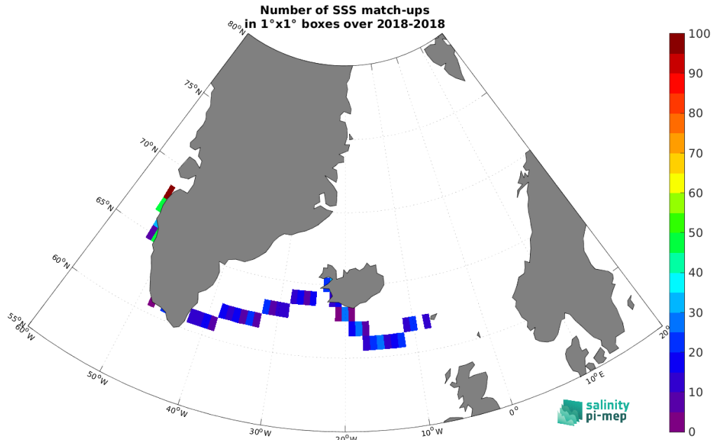
Figure 4: Number of SSS match-ups between TSG (Lauge-Koch) SSS and the SMOS and SMAP SSS L4 OI v1 - 7 Days (LOPS) SSS product for the Global Ocean Pi-MEP region over 1^\circ \times 1^\circ boxes and for the full satellite product period.
