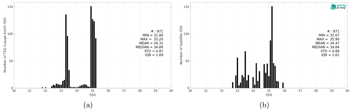
Figure 2: Histograms of SSS from TSG (Lauge-Koch) (a) and SMOS and SMAP SSS L4 OI v1 - 7 Days (LOPS) (b) considering all match-up pairs per bins of 0.1 over the Global Ocean Pi-MEP region and for the full satellite product period.
