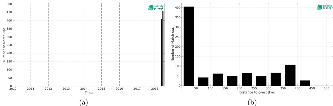
Figure 1: Number of match-ups between TSG (Lauge-Koch) and SMOS and SMAP SSS L4 OI v1 - 7 Days (LOPS) SSS as a function of time (a) and as function of the distance to coast (b) over the Global Ocean Pi-MEP region and for the full satellite product period.
