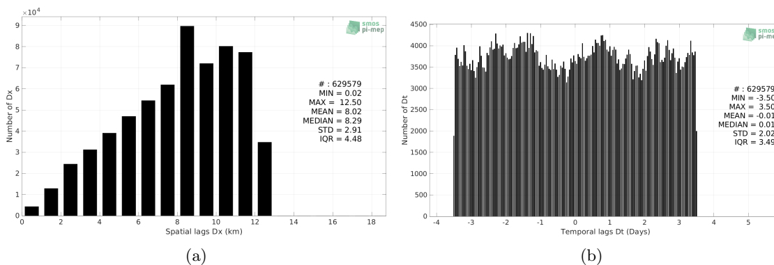
Figure 5: Histograms of the spatial (a) and temporal (b) lags between the location/time of the TSG (GOSUD-Sailing-ship) measurement and the date of the corresponding SMOS and SMAP SSS L4 OI v1 - 7 Days (LOPS) SSS pixel.
