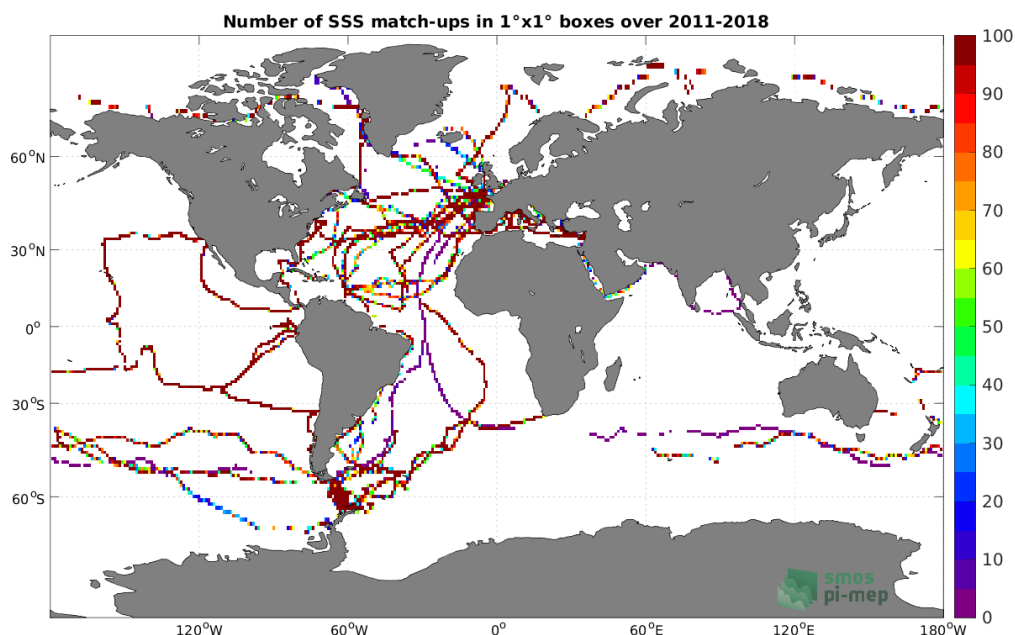
Figure 4: Number of SSS match-ups between TSG (GOSUD-Sailing-ship) SSS and the SMOS and SMAP SSS L4 OI v1 - 7 Days (LOPS) SSS product for the Global Ocean Pi-MEP region over 1^\circ \times 1^\circ boxes and for the full satellite product period.
