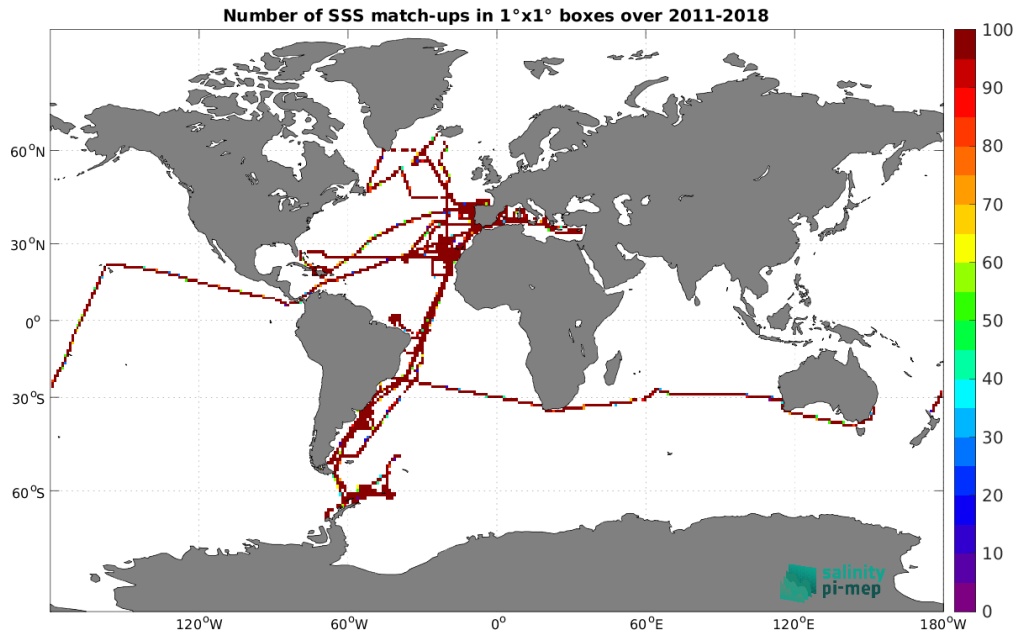
Figure 4: Number of SSS match-ups between TSG (CSIC-UTM) SSS and the SMOS and SMAP SSS L4 OI v1 - 7 Days (LOPS) SSS product for the Global Ocean Pi-MEP region over 1^\circ \times 1^\circ boxes and for the full satellite product period.
