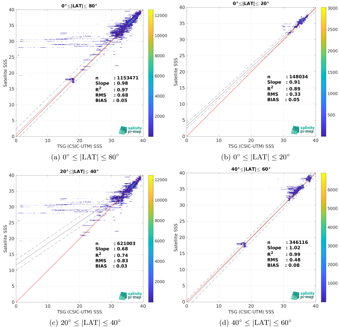
Figure 9: Contour maps of the concentration of SMOS and SMAP SSS L4 OI v1 - 7 Days (LOPS) SSS (y-axis) versus TSG (CSIC-UTM) SSS (x-axis) at match-up pairs for different latitude bands. For each plot, the red line shows x=y . The black thin and dashed lines indicate a linear fit through the data cloud and the \pm 95\% confidence levels, respectively. The number match-up pairs n , the slope and R^2 coefficient of the linear fit, the root mean square (RMS) and the mean bias between satellite and in situ data are indicated for each latitude band in each plots.
