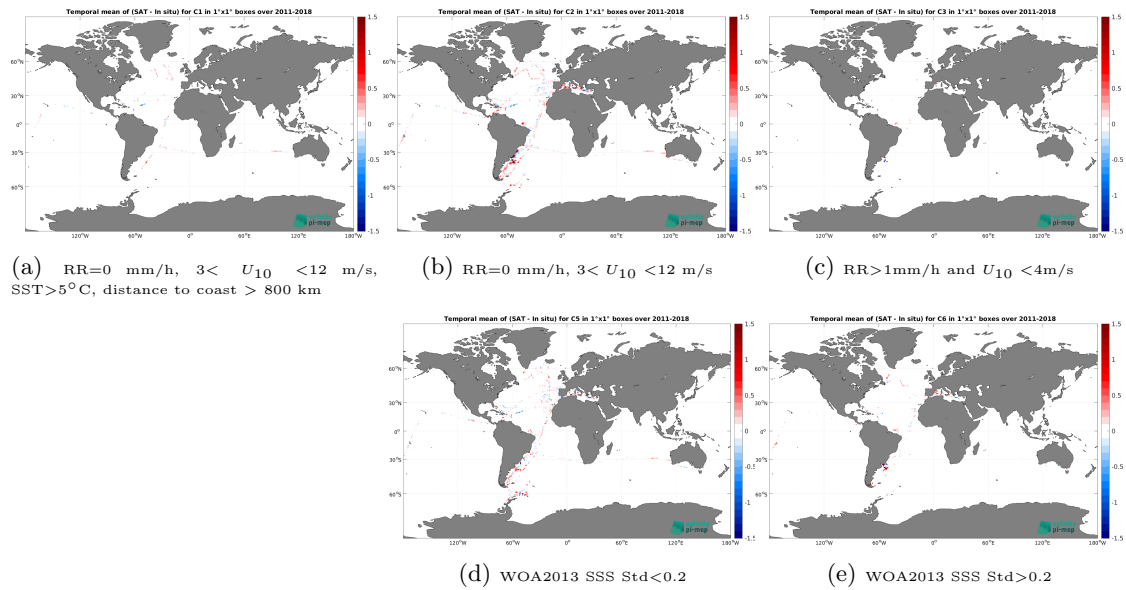
Figure 12: Temporal mean gridded over spatial boxes of size 1^\circ \times 1^\circ of \Delta SSS (SMOS and SMAP SSS L4 OI v1 - 7 Days (LOPS) - TSG (CSIC-UTM)) for 5 different subdatasets corresponding to: RR=0 mm/h, 3 < U_{10} < 12 m/s, SST > 5^\circ\text{C} , distance to coast > 800 km (a), RR=0 mm/h, 3 < U_{10} < 12 m/s (b), RR > 1\text{mm/h} and U_{10} < 4\text{m/s} (c), WOA2013 SSS Std < 0.2 (d), WOA2013 SSS Std > 0.2 (e).
