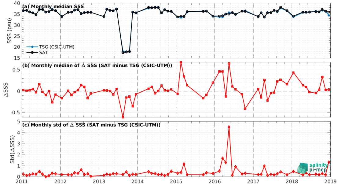
Figure 7: Time series of the monthly median SSS (top), median of \Delta\text{SSS} (Satellite - TSG (CSIC-UTM)) and Std of \Delta\text{SSS} (Satellite - TSG (CSIC-UTM)) over the Global Ocean Pi-MEP region considering all match-ups collected by the Pi-MEP.
