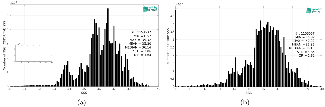
Figure 2: Histograms of SSS from TSG (CSIC-UTM) (a) and SMOS and SMAP SSS L4 OI v1 - 7 Days (LOPS) (b) considering all match-up pairs per bins of 0.1 over the Global Ocean Pi-MEP region and for the full satellite product period.
