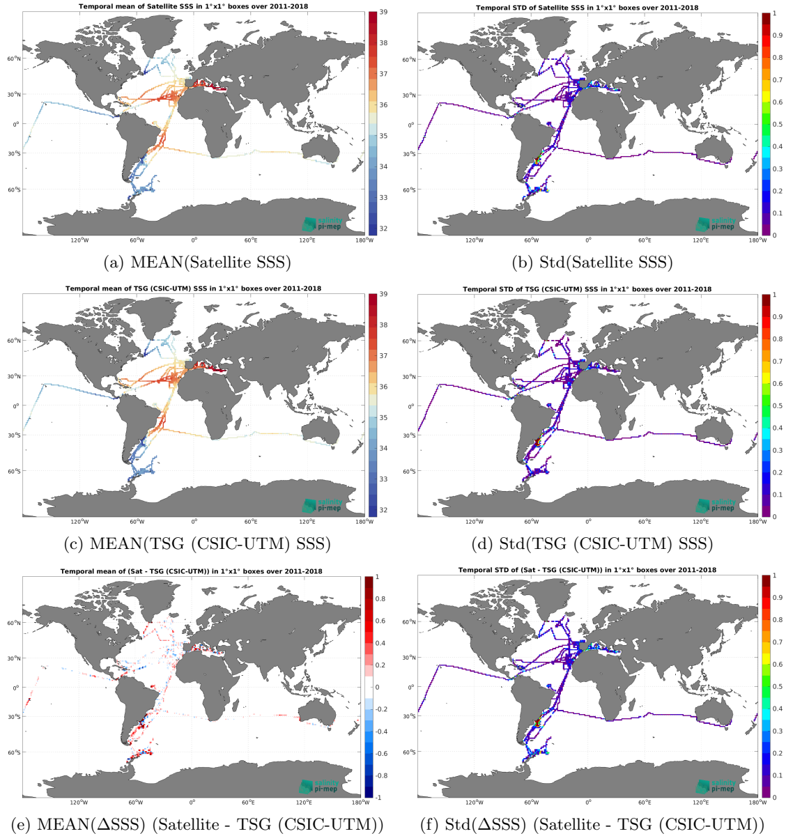
Figure 6: Temporal mean (left) and Std (right) of SSS from SMOS and SMAP SSS L4 OI v1 - 7 Days (LOPS) (top), TSG (CSIC-UTM) (middle), and of \Delta SSS (Satellite - TSG (CSIC-UTM)). Only match-up pairs are used to generate these maps.
