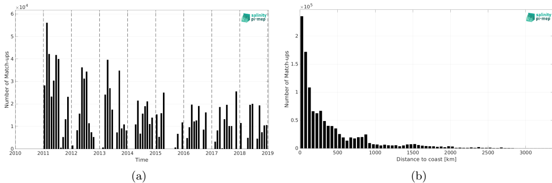
Figure 1: Number of match-ups between TSG (CSIC-UTM) and SMOS and SMAP SSS L4 OI v1 - 7 Days (LOPS) SSS as a function of time (a) and as function of the distance to coast (b) over the Global Ocean Pi-MEP region and for the full satellite product period.
