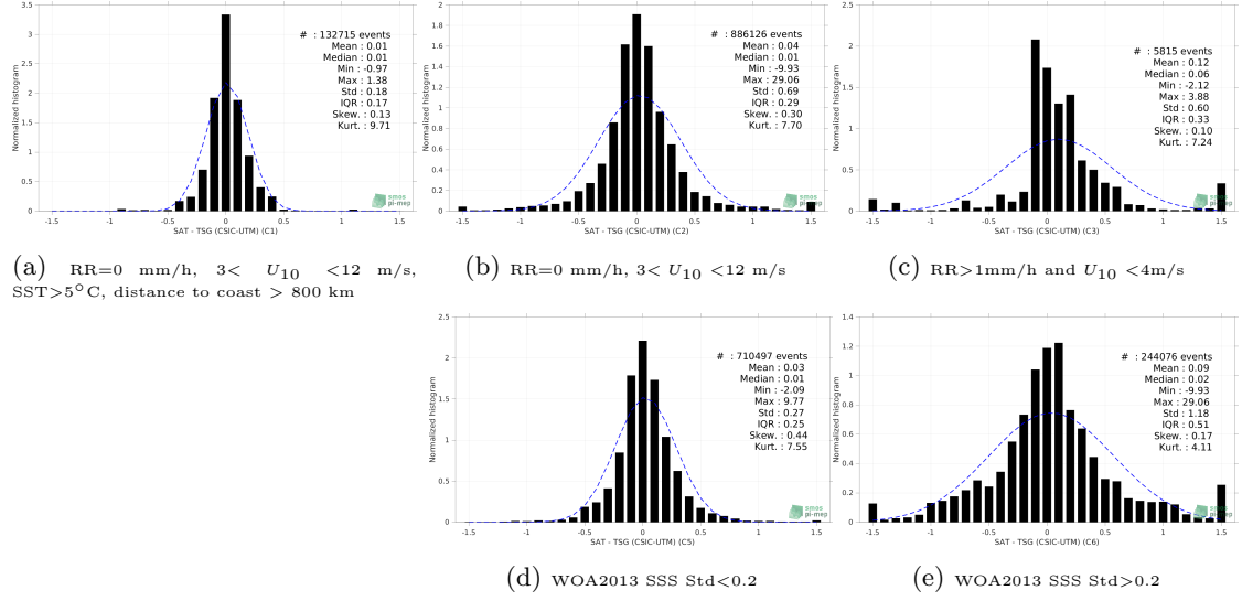
Figure 13: Normalized histogram of \Delta SSS (SMOS and SMAP SSS L4 OI v1 - 7 Days (LOPS) - TSG (CSIC-UTM)) for 5 different subdatasets corresponding to: RR=0 mm/h, 3 < U_{10} < 12 m/s, SST>5°C, distance to coast > 800 km (a), RR=0 mm/h, 3 < U_{10} < 12 m/s (b), RR>1mm/h and U_{10} < 4 m/s (c), WOA2013 SSS Std<0.2 (d), WOA2013 SSS Std>0.2 (e).
