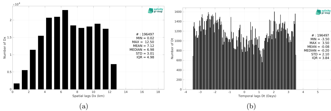
Figure 5: Histograms of the spatial (a) and temporal (b) lags between the location/time of the TSG (Amundsen) measurement and the date of the corresponding SMOS and SMAP SSS L4 OI v1 - 7 Days (LOPS) SSS pixel.
