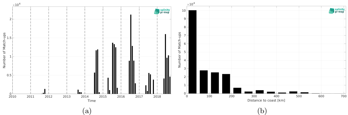
Figure 1: Number of match-ups between TSG (Amundsen) and SMOS and SMAP SSS L4 OI v1 - 7 Days (LOPS) SSS as a function of time (a) and as function of the distance to coast (b) over the Global Ocean Pi-MEP region and for the full satellite product period.
