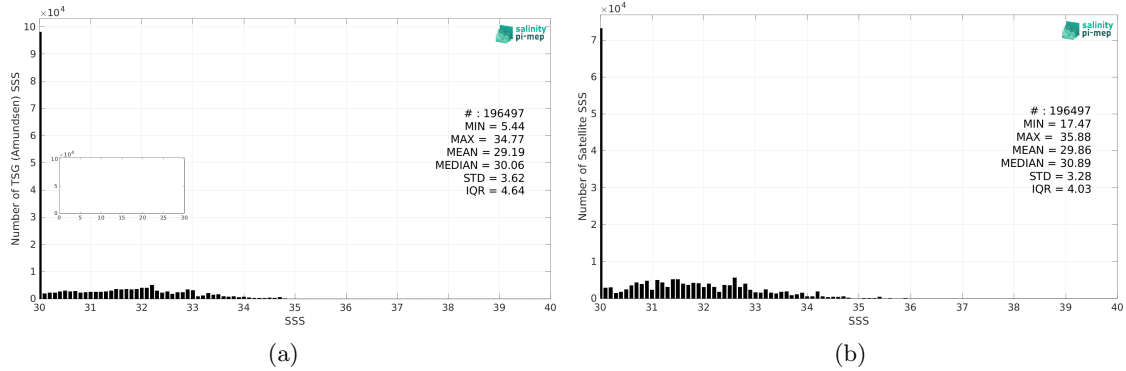
Figure 2: Histograms of SSS from TSG (Amundsen) (a) and SMOS and SMAP SSS L4 OI v1 - 7 Days (LOPS) (b) considering all match-up pairs per bins of 0.1 over the Global Ocean Pi-MEP region and for the full satellite product period.
