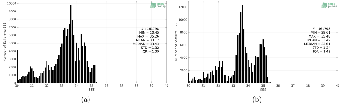
Figure 2: Histograms of SSS from Sairdrone (a) and SMOS and SMAP SSS L4 OI v1 - 7 Days (LOPS) (b) considering all match-up pairs per bins of 0.1 over the Global Ocean Pi-MEP region and for the full satellite product period.
