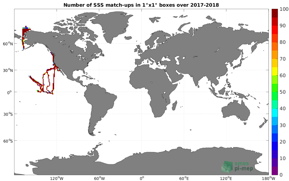
Figure 4: Number of SSS match-ups between Saildrone SSS and the SMOS and SMAP SSS L4 OI v1 - 7 Days (LOPS) SSS product for the Global Ocean Pi-MEP region over 1°×1° boxes and for the full satellite product period.
