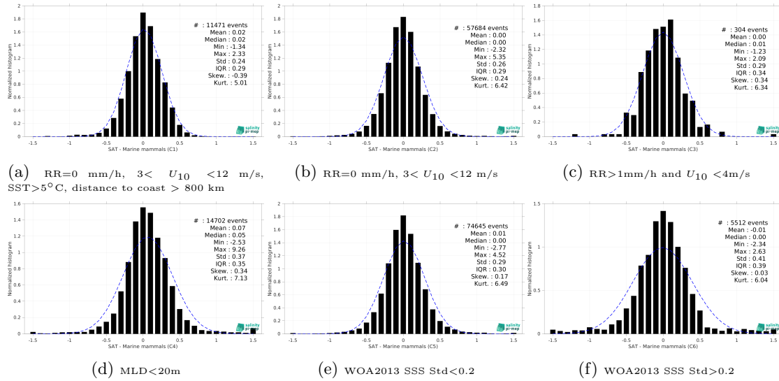
Figure 13: Normalized histogram of \Delta\text{SSS} (SMOS and SMAP SSS L4 OI v1 - 7 Days (LOPS) - Marine mammals) for 6 different subdatasets corresponding to: RR=0 mm/h, 3 < U_{10} < 12 m/s, SST>5°C, distance to coast > 800 km (a), RR=0 mm/h, 3 < U_{10} < 12 m/s (b), RR>1mm/h and U_{10} < 4 m/s (c), MLD<20m (d), WOA2013 SSS Std<0.2 (e), WOA2013 SSS Std>0.2 (f).
