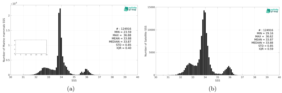
Figure 2: Histograms of SSS from Marine mammals (a) and SMOS and SMAP SSS L4 OI v1 - 7 Days (LOPS) (b) considering all match-up pairs per bins of 0.1 over the Global Ocean Pi-MEP region and for the full satellite product period.
